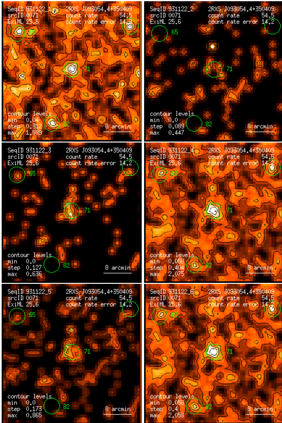
Figure 71: RASS 931122: detection 0071: band rate images, Gaussian filter: (1) PSPC channels 11 – 41, (2) 52 – 90, (3) 91 – 201, (4) 11 – 235, (5) 52 – 201, (6) 11 – 201. Broad band rates in counts/ks. Band rate contour levels in counts/ks/arcmin 2 .
