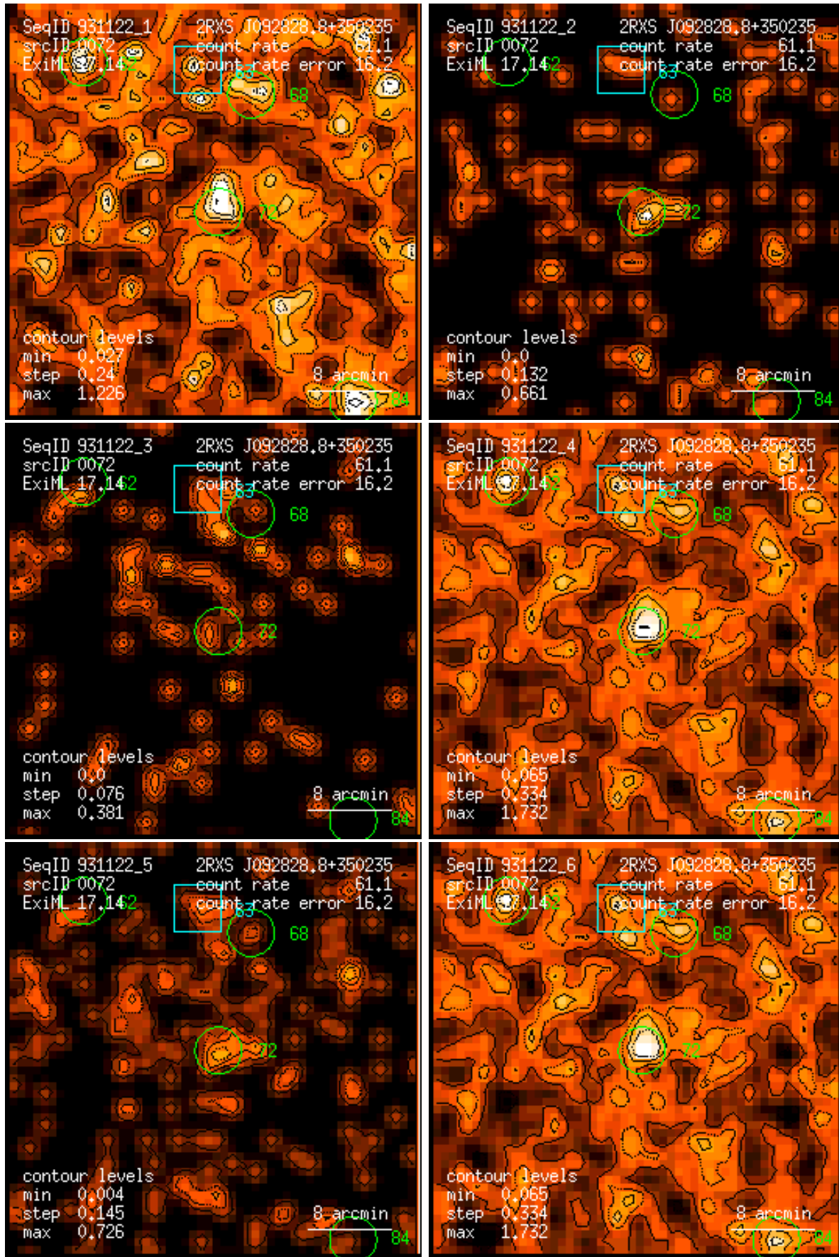
Figure 72: RASS 931122: detection 0072: band rate images, Gaussian filter: (1) PSPC channels 11 – 41, (2) 52 – 90, (3) 91 – 201, (4) 11 – 235, (5) 52 – 201, (6) 11 – 201. Broad band rates in counts/ks. Band rate contour levels in counts/ks/arcmin 2 .
