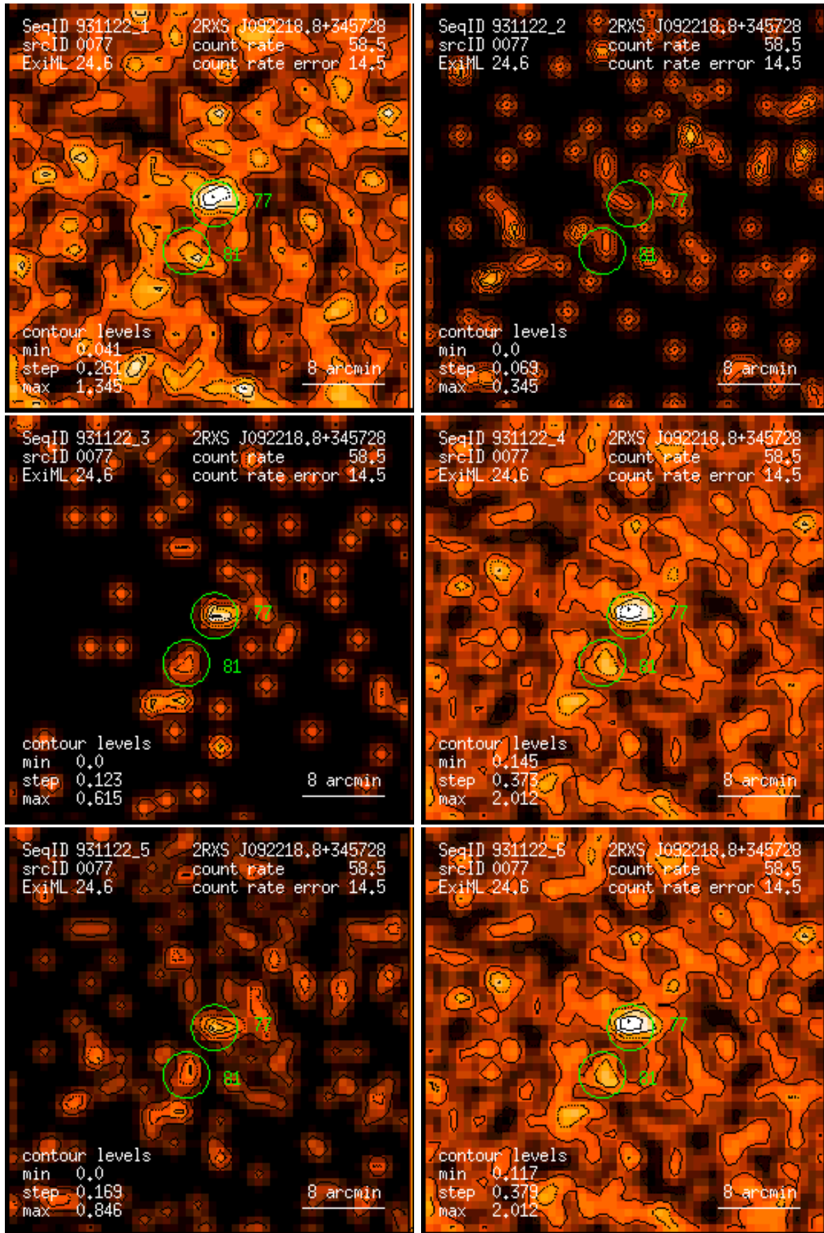
Figure 77: RASS 931122: detection 0077: band rate images, Gaussian filter: (1) PSPC channels 11 – 41, (2) 52 – 90, (3) 91 – 201, (4) 11 – 235, (5) 52 – 201, (6) 11 – 201. Broad band rates in counts/ks. Band rate contour levels in counts/ks/arcmin 2 .
