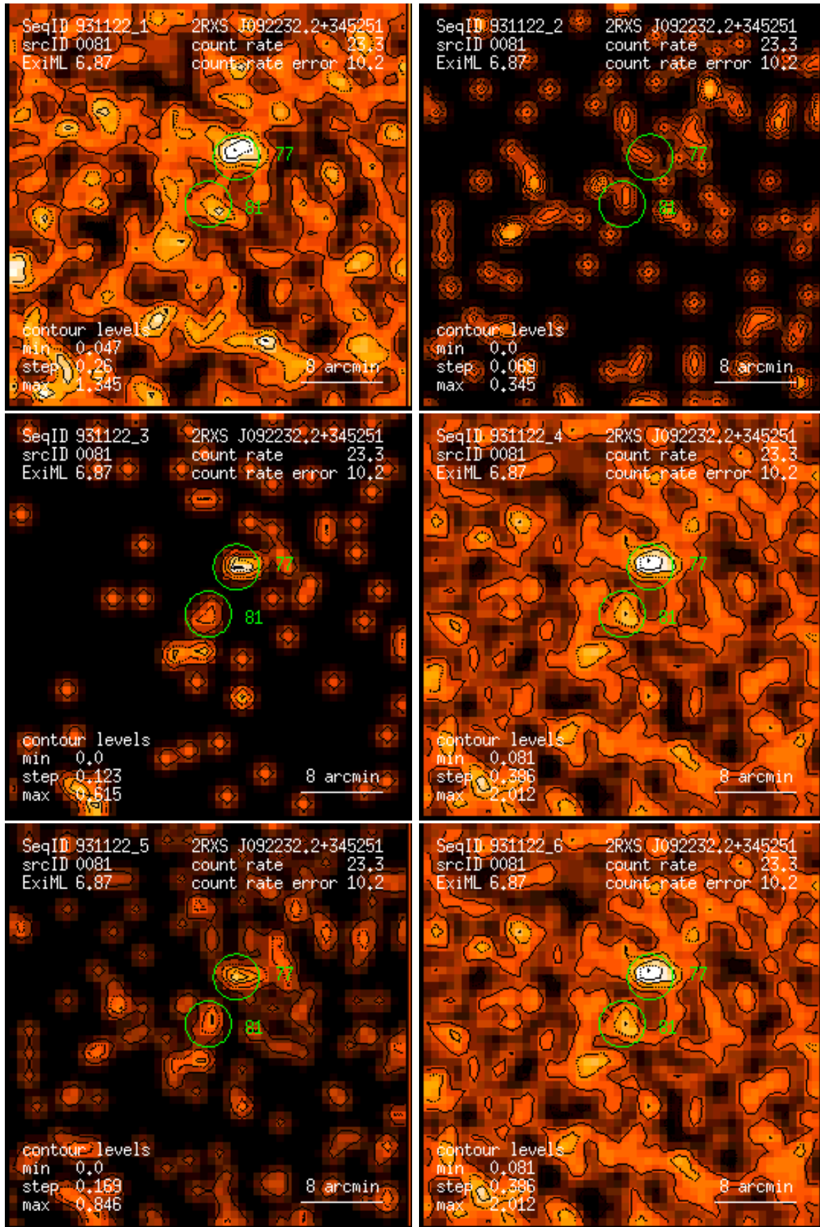
Figure 81: RASS 931122: detection 0081: band rate images, Gaussian filter: (1) PSPC channels 11 – 41, (2) 52 – 90, (3) 91 – 201, (4) 11 – 235, (5) 52 – 201, (6) 11 – 201. Broad band rates in counts/ks. Band rate contour levels in counts/ks/arcmin 2 .
