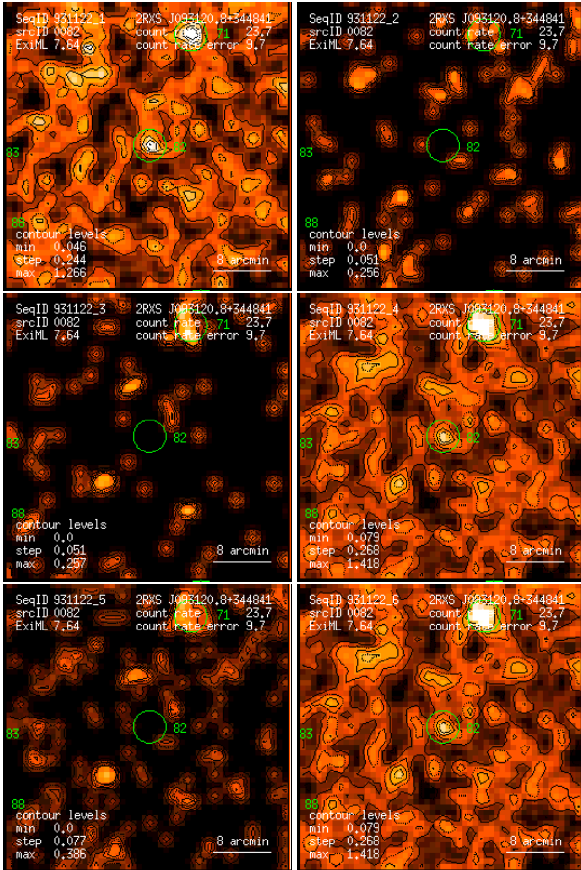
Figure 82: RASS 931122: detection 0082: band rate images, Gaussian filter: (1) PSPC channels 11 – 41, (2) 52 – 90, (3) 91 – 201, (4) 11 – 235, (5) 52 – 201, (6) 11 – 201. Broad band rates in counts/ks. Band rate contour levels in counts/ks/arcmin 2 .
