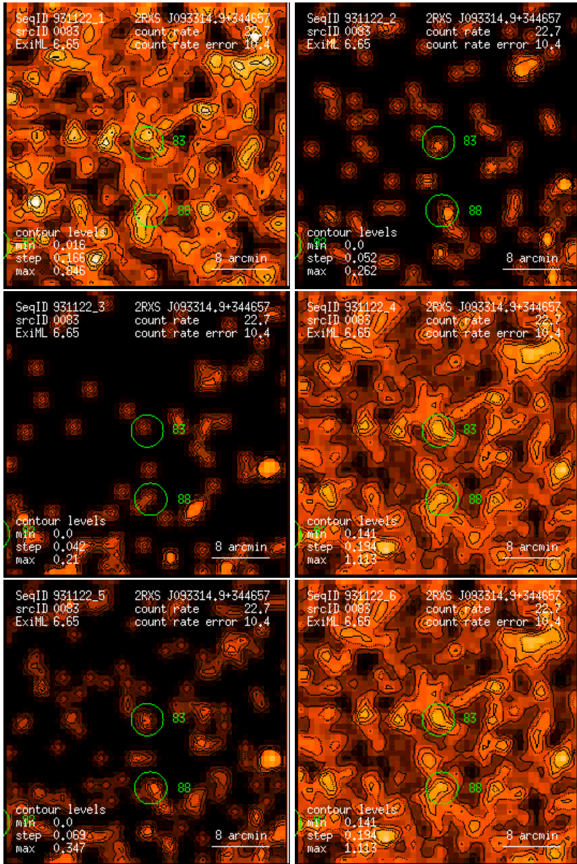
Figure 83: RASS 931122: detection 0083: band rate images, Gaussian filter: (1) PSPC channels 11 – 41, (2) 52 – 90, (3) 91 – 201, (4) 11 – 235, (5) 52 – 201, (6) 11 – 201. Broad band rates in counts/ks. Band rate contour levels in counts/ks/arcmin 2 .
