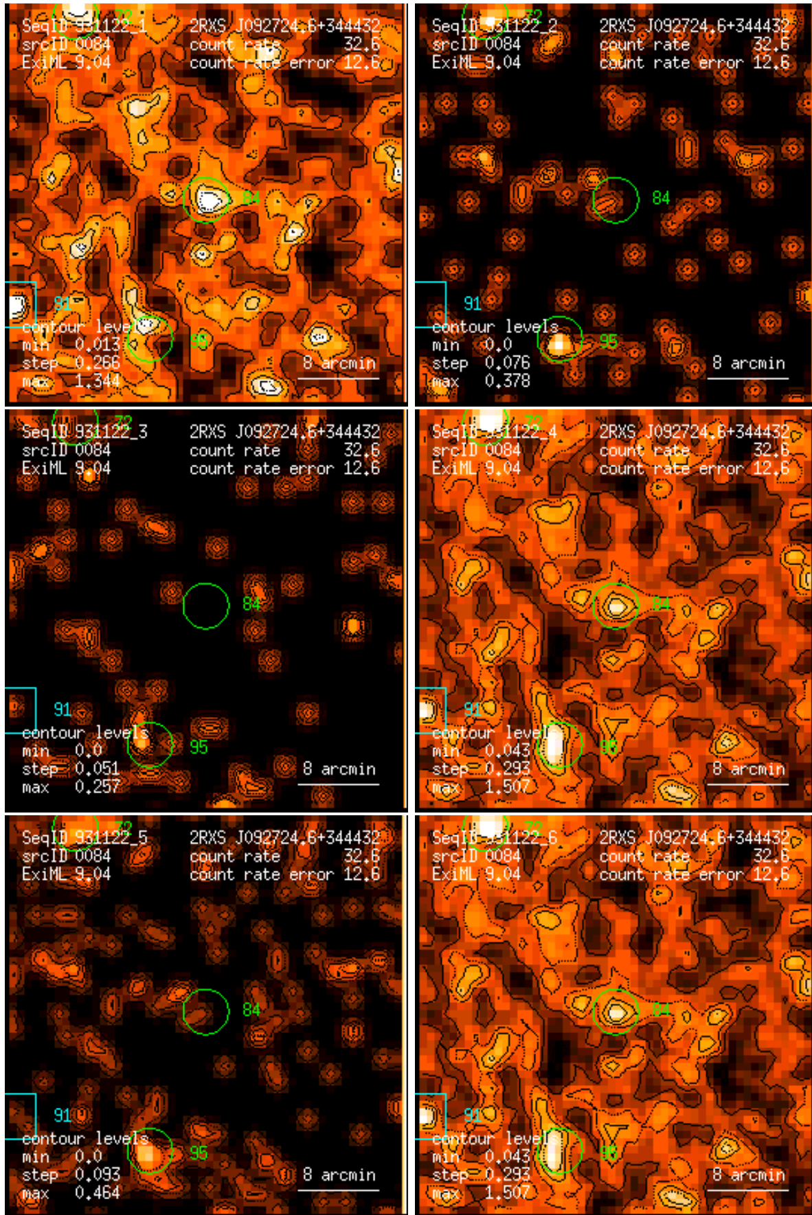
Figure 84: RASS 931122: detection 0084: band rate images, Gaussian filter: (1) PSPC channels 11 – 41, (2) 52 – 90, (3) 91 – 201, (4) 11 – 235, (5) 52 – 201, (6) 11 – 201. Broad band rates in counts/ks. Band rate contour levels in counts/ks/arcmin 2 .
