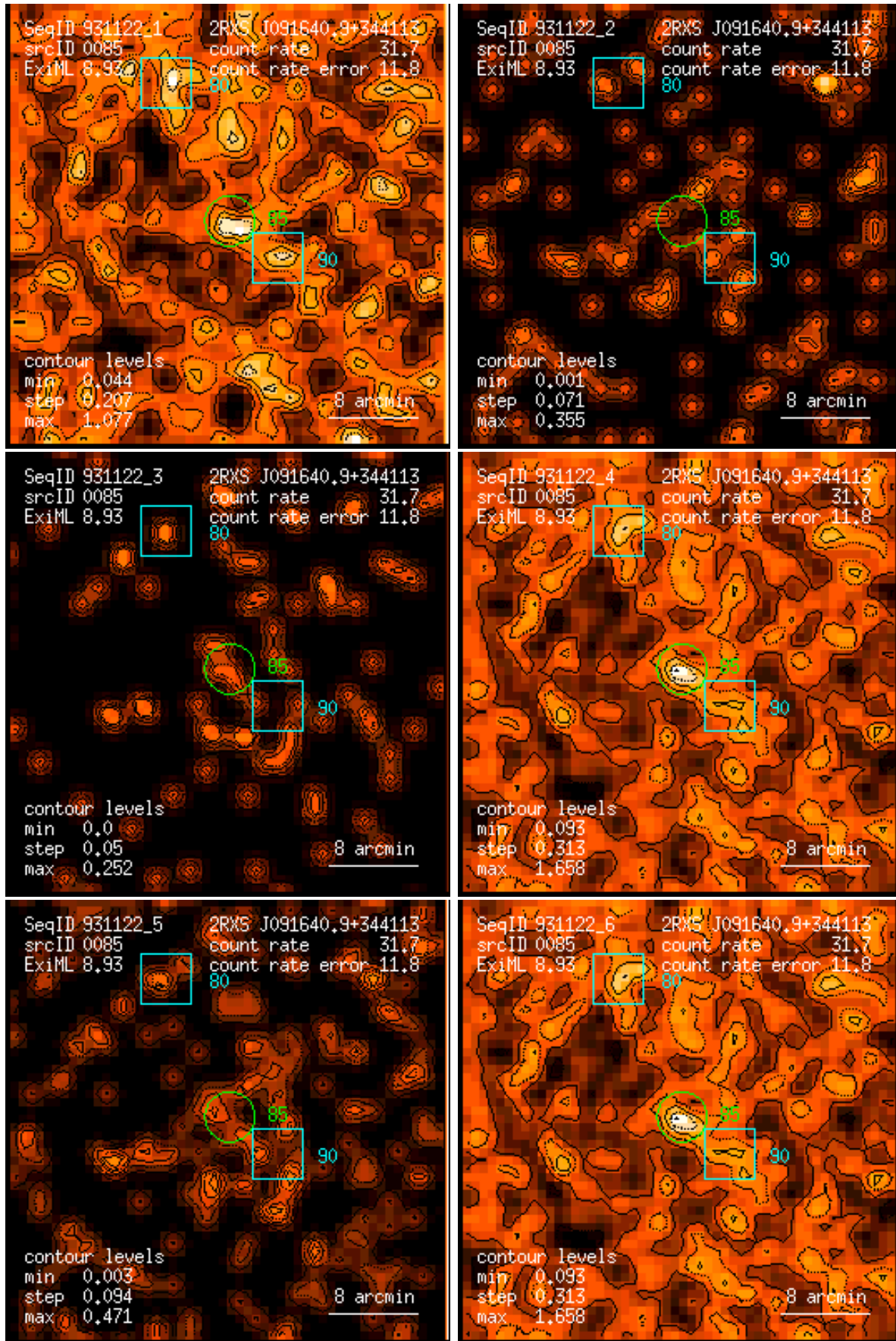
Figure 85: RASS 931122: detection 0085: band rate images, Gaussian filter: (1) PSPC channels 11 – 41, (2) 52 – 90, (3) 91 – 201, (4) 11 – 235, (5) 52 – 201, (6) 11 – 201. Broad band rates in counts/ks. Band rate contour levels in counts/ks/arcmin 2 .
