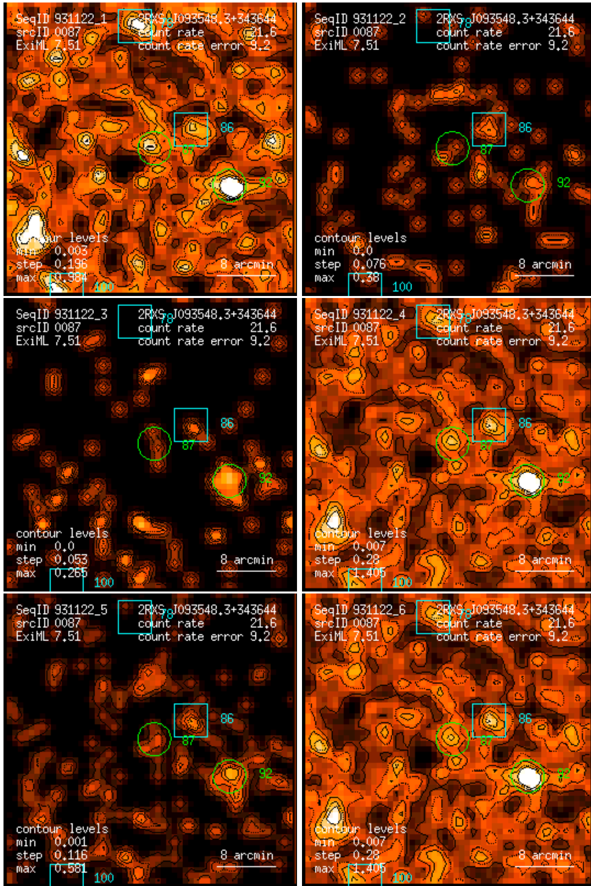
Figure 87: RASS 931122: detection 0087: band rate images, Gaussian filter: (1) PSPC channels 11 – 41, (2) 52 – 90, (3) 91 – 201, (4) 11 – 235, (5) 52 – 201, (6) 11 – 201. Broad band rates in counts/ks. Band rate contour levels in counts/ks/arcmin 2 .
