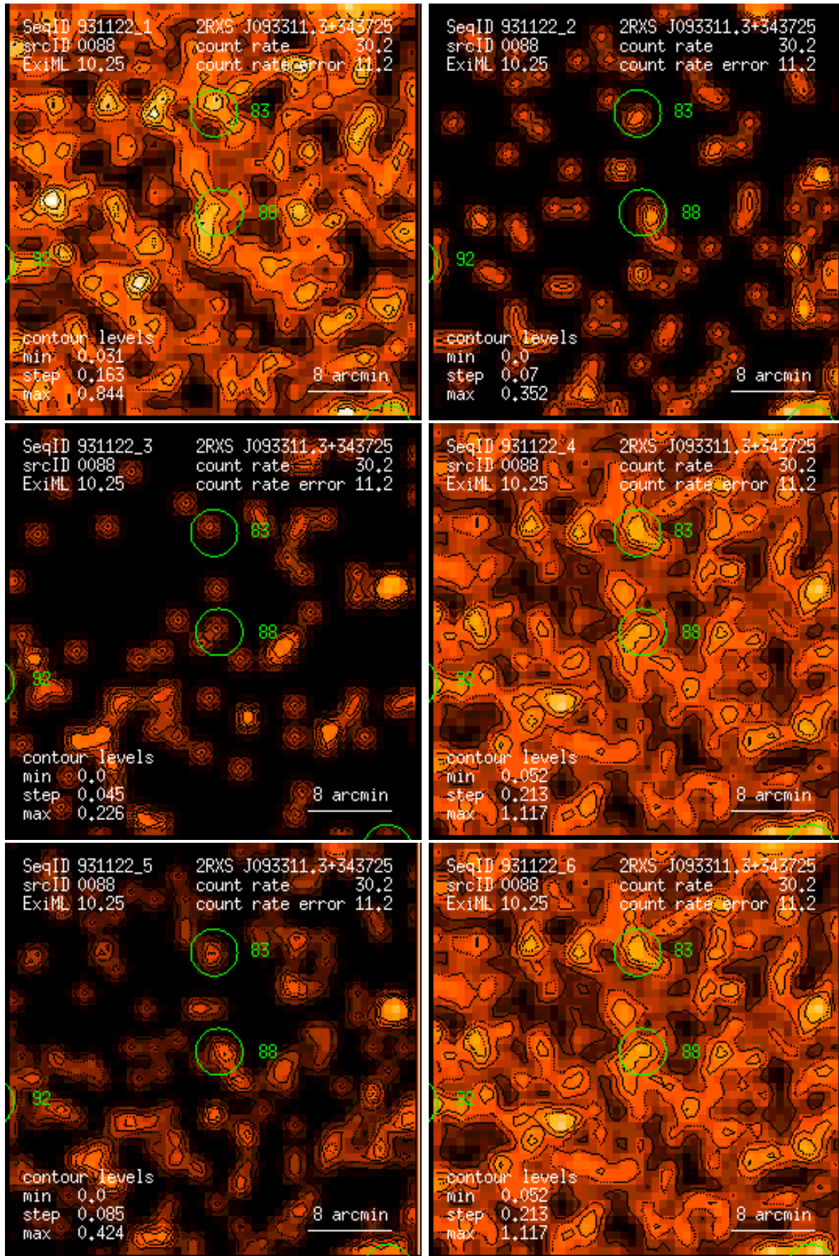
Figure 88: RASS 931122: detection 0088: band rate images, Gaussian filter: (1) PSPC channels 11 – 41, (2) 52 – 90, (3) 91 – 201, (4) 11 – 235, (5) 52 – 201, (6) 11 – 201. Broad band rates in counts/ks. Band rate contour levels in counts/ks/arcmin 2 .
