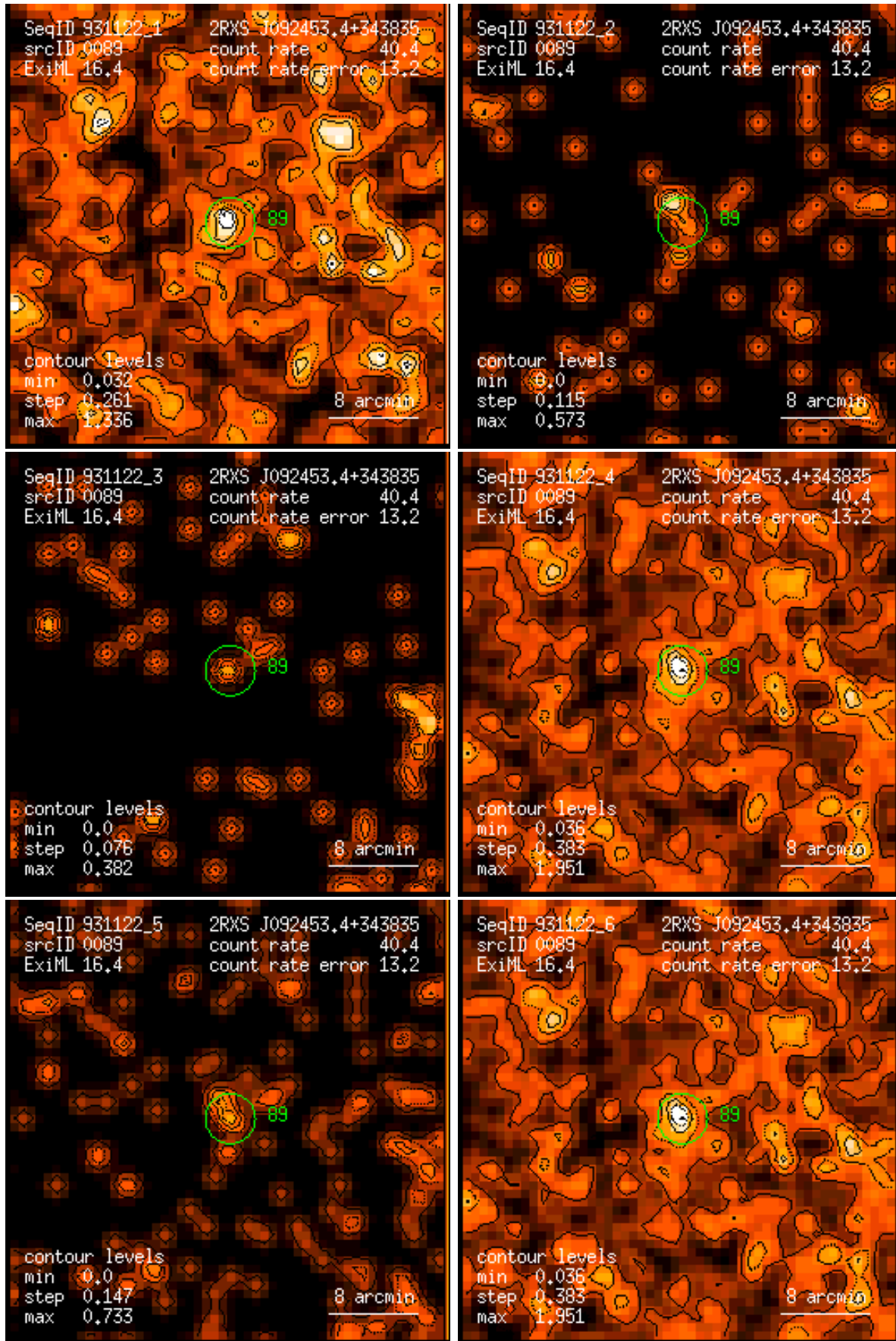
Figure 89: RASS 931122: detection 0089: band rate images, Gaussian filter: (1) PSPC channels 11 – 41, (2) 52 – 90, (3) 91 – 201, (4) 11 – 235, (5) 52 – 201, (6) 11 – 201. Broad band rates in counts/ks. Band rate contour levels in counts/ks/arcmin 2 .
