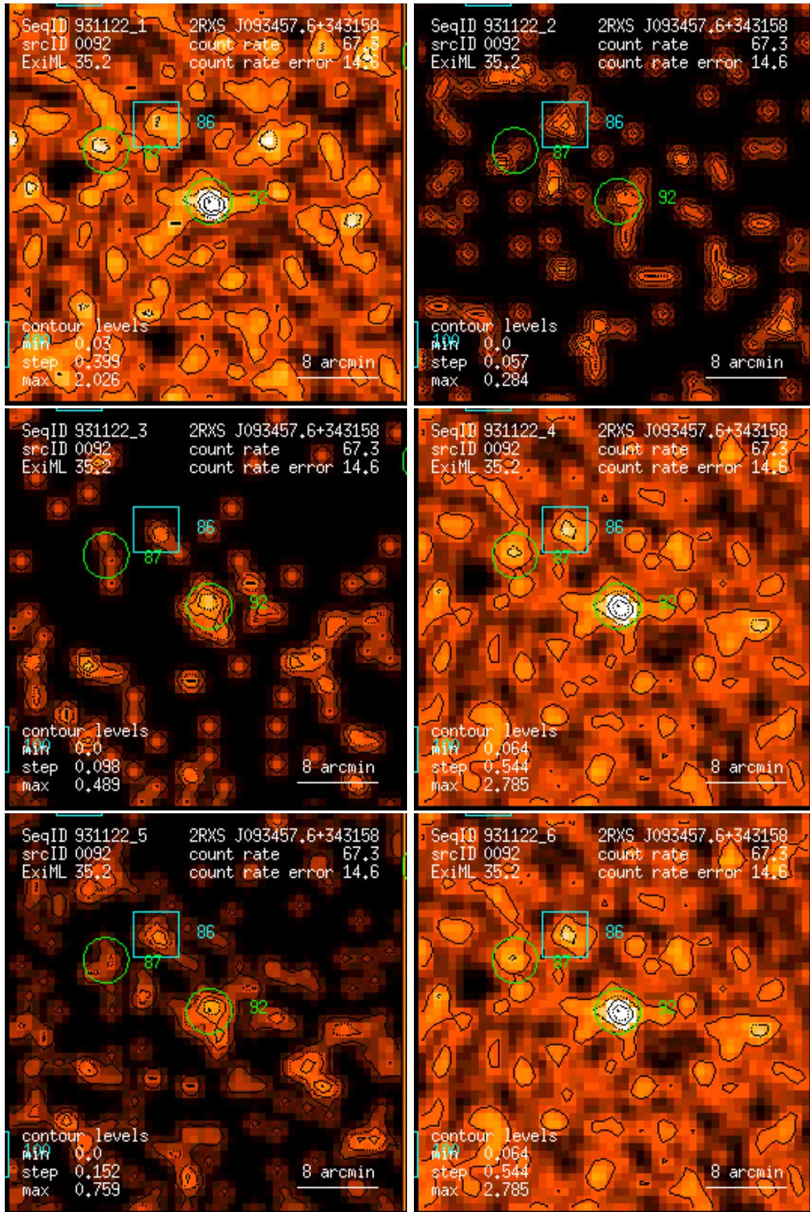
Figure 92: RASS 931122: detection 0092: band rate images, Gaussian filter: (1) PSPC channels 11 – 41, (2) 52 – 90, (3) 91 – 201, (4) 11 – 235, (5) 52 – 201, (6) 11 – 201. Broad band rates in counts/ks. Band rate contour levels in counts/ks/arcmin 2 .
