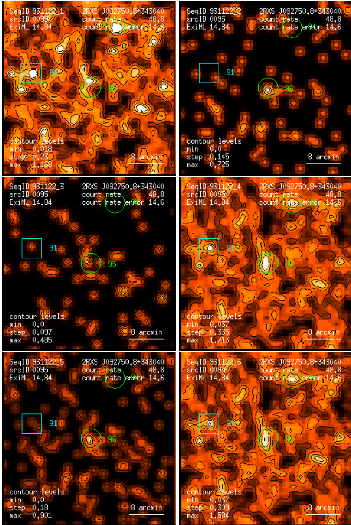
Figure 95: RASS 931122: detection 0095: band rate images, Gaussian filter: (1) PSPC channels 11 – 41, (2) 52 – 90, (3) 91 – 201, (4) 11 – 235, (5) 52 – 201, (6) 11 – 201. Broad band rates in counts/ks. Band rate contour levels in counts/ks/arcmin 2 .
