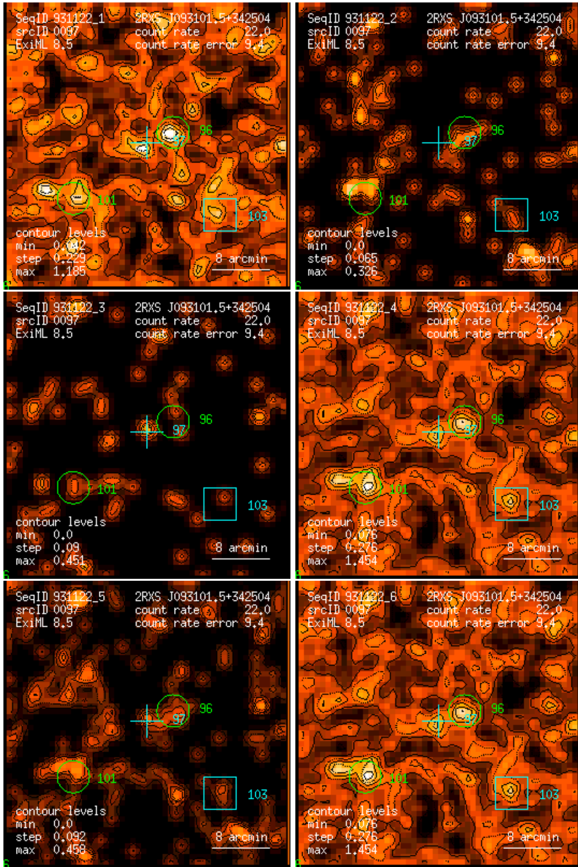
Figure 97: RASS 931122: detection 0097: band rate images, Gaussian filter: (1) PSPC channels 11 – 41, (2) 52 – 90, (3) 91 – 201, (4) 11 – 235, (5) 52 – 201, (6) 11 – 201. Broad band rates in counts/ks. Band rate contour levels in counts/ks/arcmin 2 .
