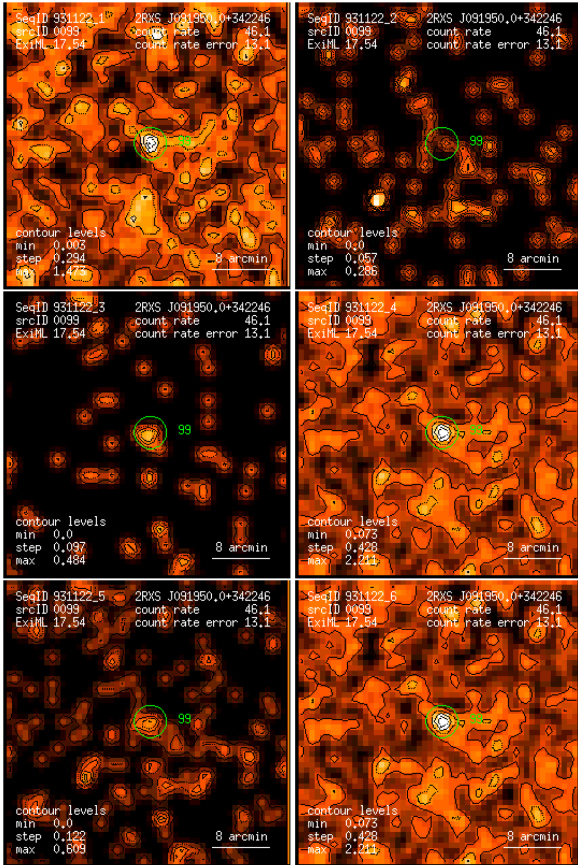
Figure 99: RASS 931122: detection 0099: band rate images, Gaussian filter: (1) PSPC channels 11 – 41, (2) 52 – 90, (3) 91 – 201, (4) 11 – 235, (5) 52 – 201, (6) 11 – 201. Broad band rates in counts/ks. Band rate contour levels in counts/ks/arcmin 2 .
