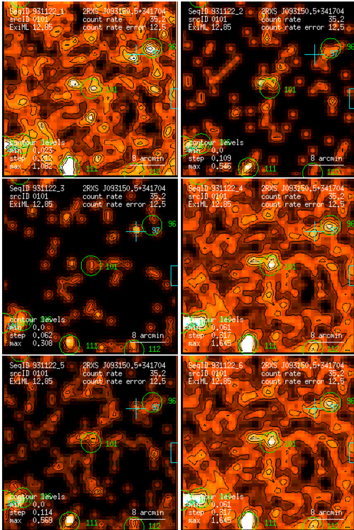
Figure 101: RASS 931122: detection 0101: band rate images, Gaussian filter: (1) PSPC channels 11 – 41, (2) 52 – 90, (3) 91 – 201, (4) 11 – 235, (5) 52 – 201, (6) 11 – 201. Broad band rates in counts/ks. Band rate contour levels in counts/ks/arcmin 2 .
