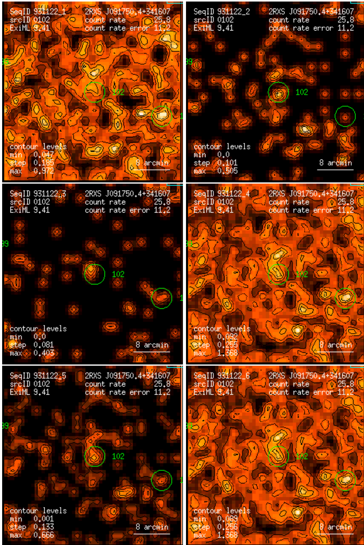
Figure 102: RASS 931122: detection 0102: band rate images, Gaussian filter: (1) PSPC channels 11 – 41, (2) 52 – 90, (3) 91 – 201, (4) 11 – 235, (5) 52 – 201, (6) 11 – 201. Broad band rates in counts/ks. Band rate contour levels in counts/ks/arcmin 2 .
