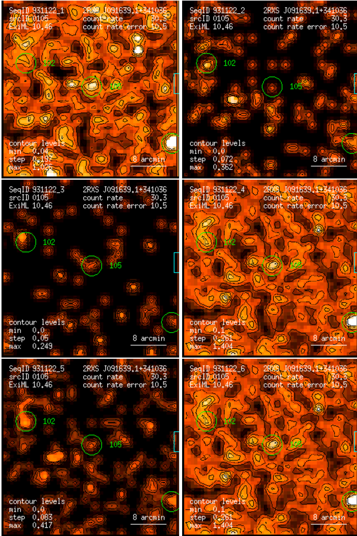
Figure 105: RASS 931122: detection 0105: band rate images, Gaussian filter: (1) PSPC channels 11 – 41, (2) 52 – 90, (3) 91 – 201, (4) 11 – 235, (5) 52 – 201, (6) 11 – 201. Broad band rates in counts/ks. Band rate contour levels in counts/ks/arcmin 2 .
