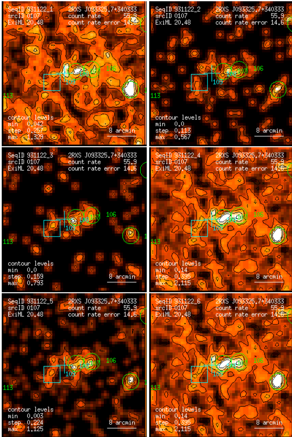
Figure 107: RASS 931122: detection 0107: band rate images, Gaussian filter: (1) PSPC channels 11 – 41, (2) 52 – 90, (3) 91 – 201, (4) 11 – 235, (5) 52 – 201, (6) 11 – 201. Broad band rates in counts/ks. Band rate contour levels in counts/ks/arcmin 2 .
