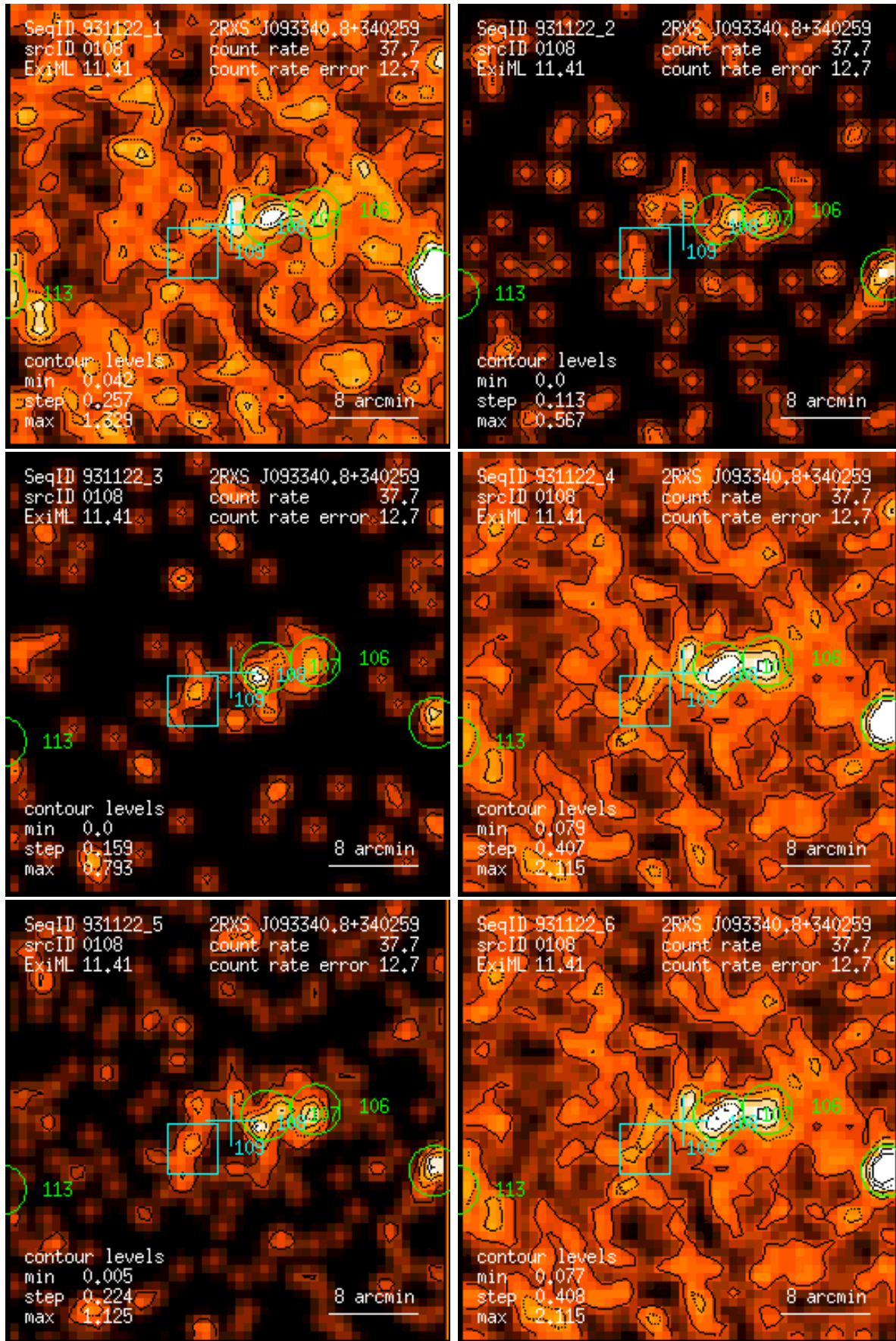
Figure 108: RASS 931122: detection 0108: band rate images, Gaussian filter: (1) PSPC channels 11 – 41, (2) 52 – 90, (3) 91 – 201, (4) 11 – 235, (5) 52 – 201, (6) 11 – 201. Broad band rates in counts/ks. Band rate contour levels in counts/ks/arcmin 2 .
