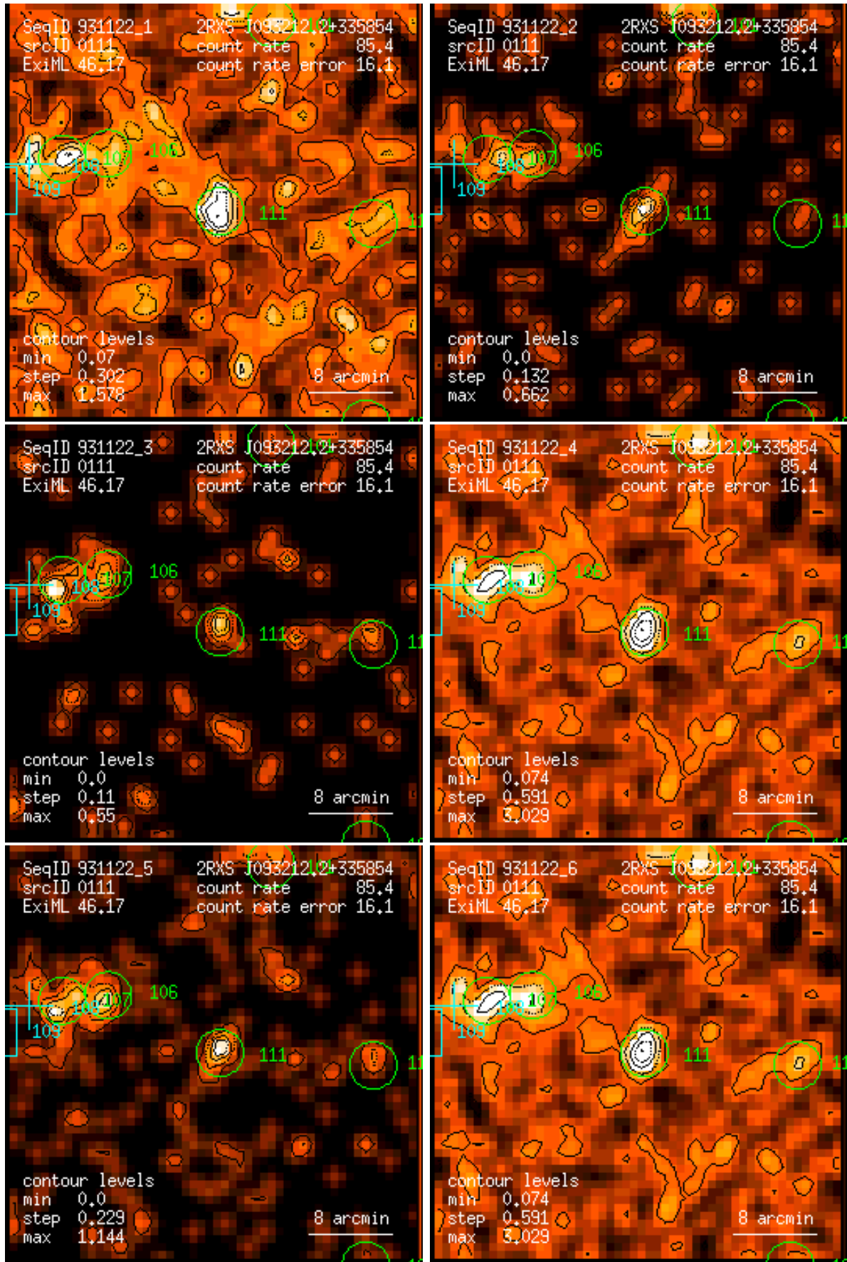
Figure 111: RASS 931122: detection 0111: band rate images, Gaussian filter: (1) PSPC channels 11 – 41, (2) 52 – 90, (3) 91 – 201, (4) 11 – 235, (5) 52 – 201, (6) 11 – 201. Broad band rates in counts/ks. Band rate contour levels in counts/ks/arcmin 2 .
