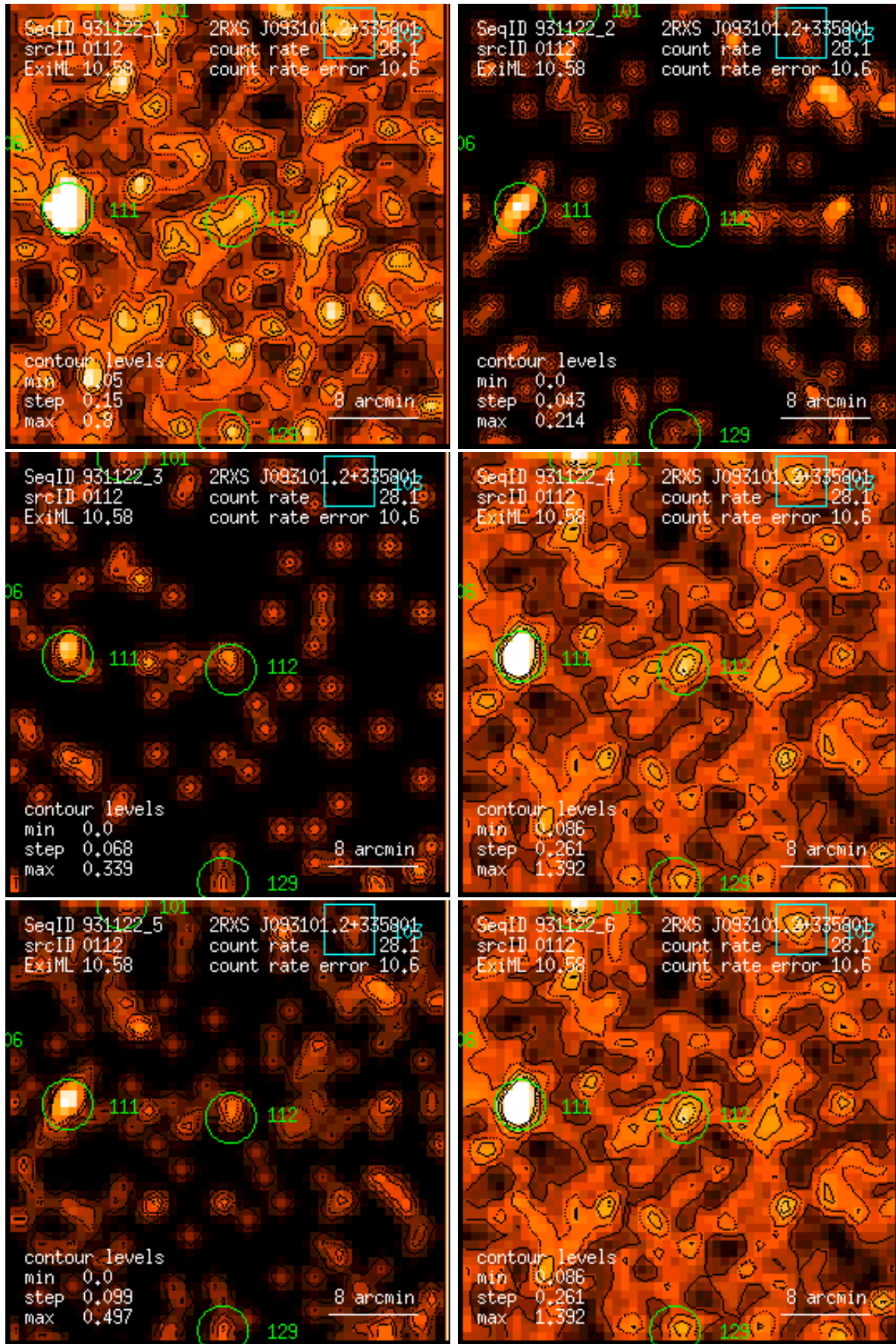
Figure 112: RASS 931122: detection 0112: band rate images, Gaussian filter: (1) PSPC channels 11 – 41, (2) 52 – 90, (3) 91 – 201, (4) 11 – 235, (5) 52 – 201, (6) 11 – 201. Broad band rates in counts/ks. Band rate contour levels in counts/ks/arcmin 2 .
