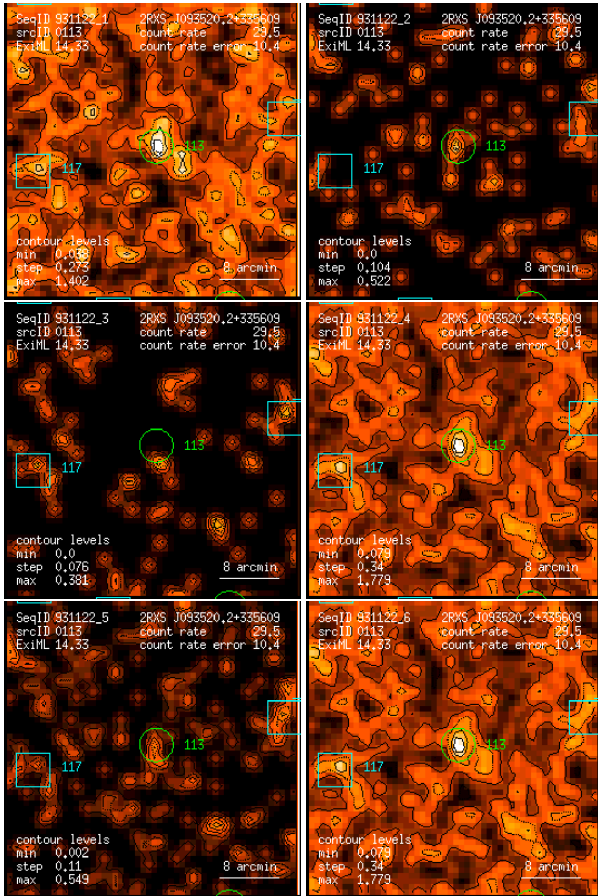
Figure 113: RASS 931122: detection 0113: band rate images, Gaussian filter: (1) PSPC channels 11 – 41, (2) 52 – 90, (3) 91 – 201, (4) 11 – 235, (5) 52 – 201, (6) 11 – 201. Broad band rates in counts/ks. Band rate contour levels in counts/ks/arcmin 2 .
