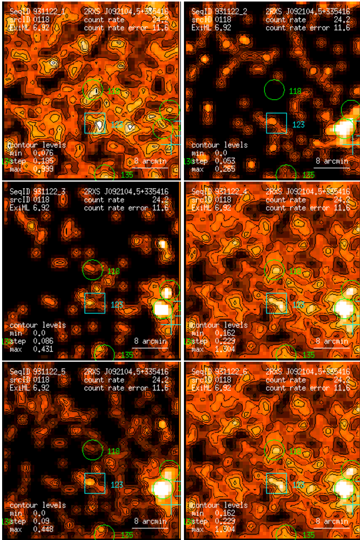
Figure 118: RASS 931122: detection 0118: band rate images, Gaussian filter: (1) PSPC channels 11 – 41, (2) 52 – 90, (3) 91 – 201, (4) 11 – 235, (5) 52 – 201, (6) 11 – 201. Broad band rates in counts/ks. Band rate contour levels in counts/ks/arcmin 2 .
