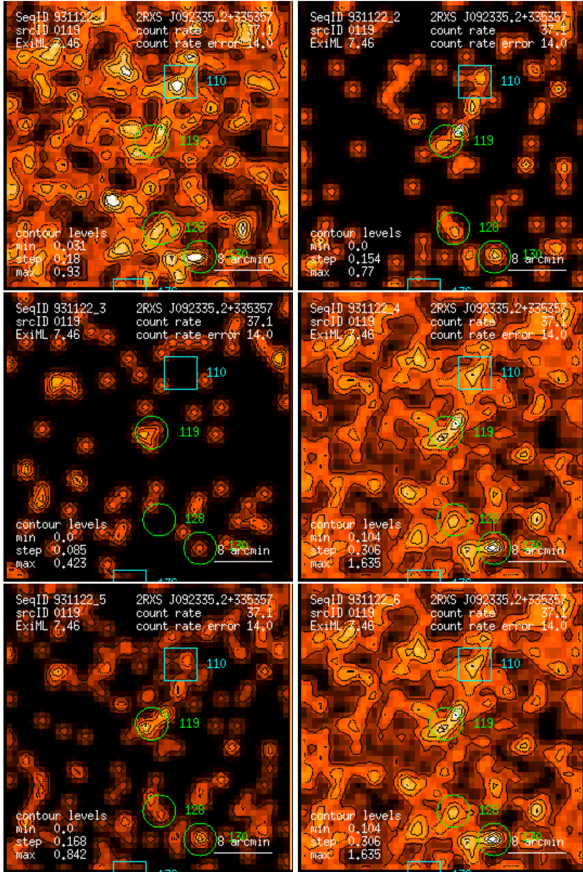
Figure 119: RASS 931122: detection 0119: band rate images, Gaussian filter: (1) PSPC channels 11 – 41, (2) 52 – 90, (3) 91 – 201, (4) 11 – 235, (5) 52 – 201, (6) 11 – 201. Broad band rates in counts/ks. Band rate contour levels in counts/ks/arcmin 2 .
