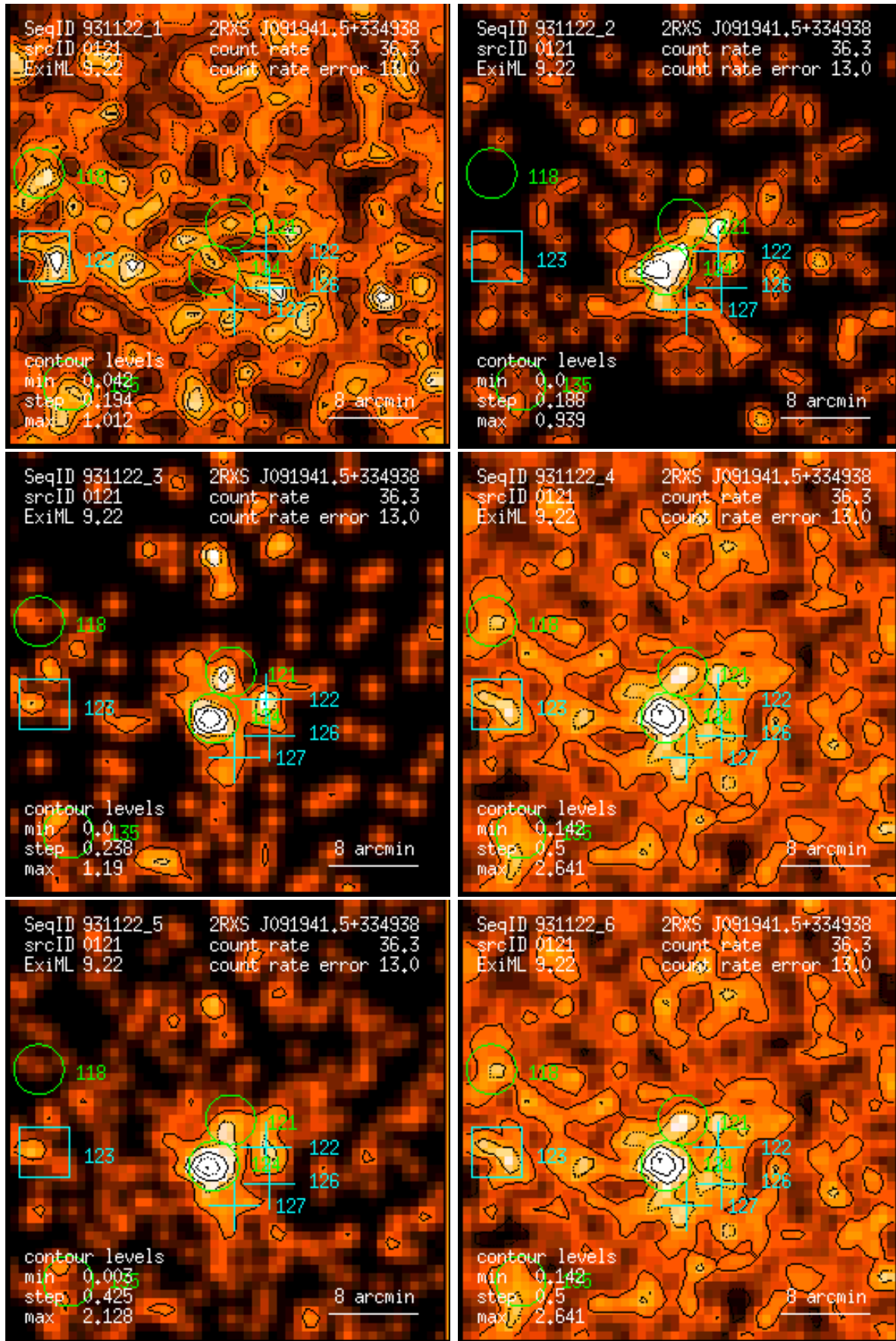
Figure 121: RASS 931122: detection 0121: band rate images, Gaussian filter: (1) PSPC channels 11 – 41, (2) 52 – 90, (3) 91 – 201, (4) 11 – 235, (5) 52 – 201, (6) 11 – 201. Broad band rates in counts/ks. Band rate contour levels in counts/ks/arcmin 2 .
