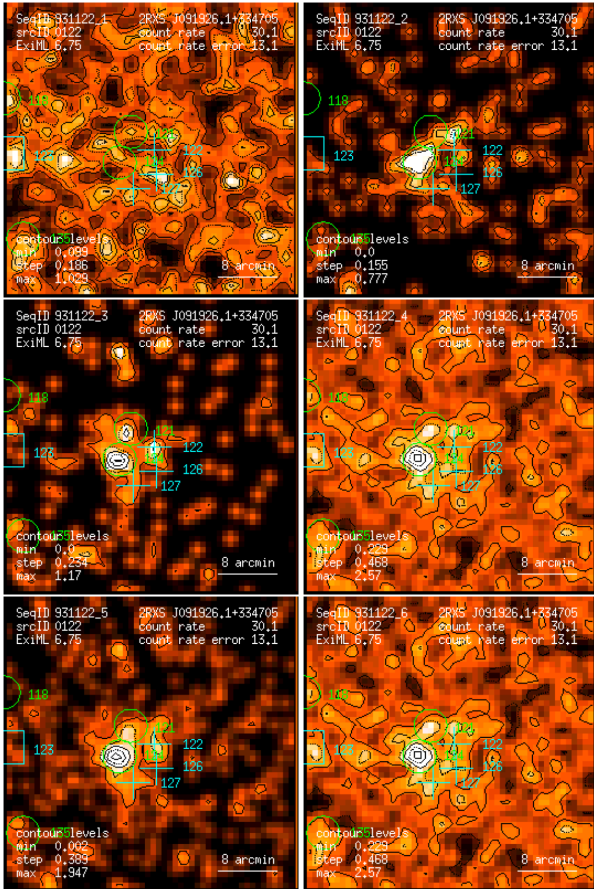
Figure 122: RASS 931122: detection 0122: band rate images, Gaussian filter: (1) PSPC channels 11 – 41, (2) 52 – 90, (3) 91 – 201, (4) 11 – 235, (5) 52 – 201, (6) 11 – 201. Broad band rates in counts/ks. Band rate contour levels in counts/ks/arcmin 2 .
