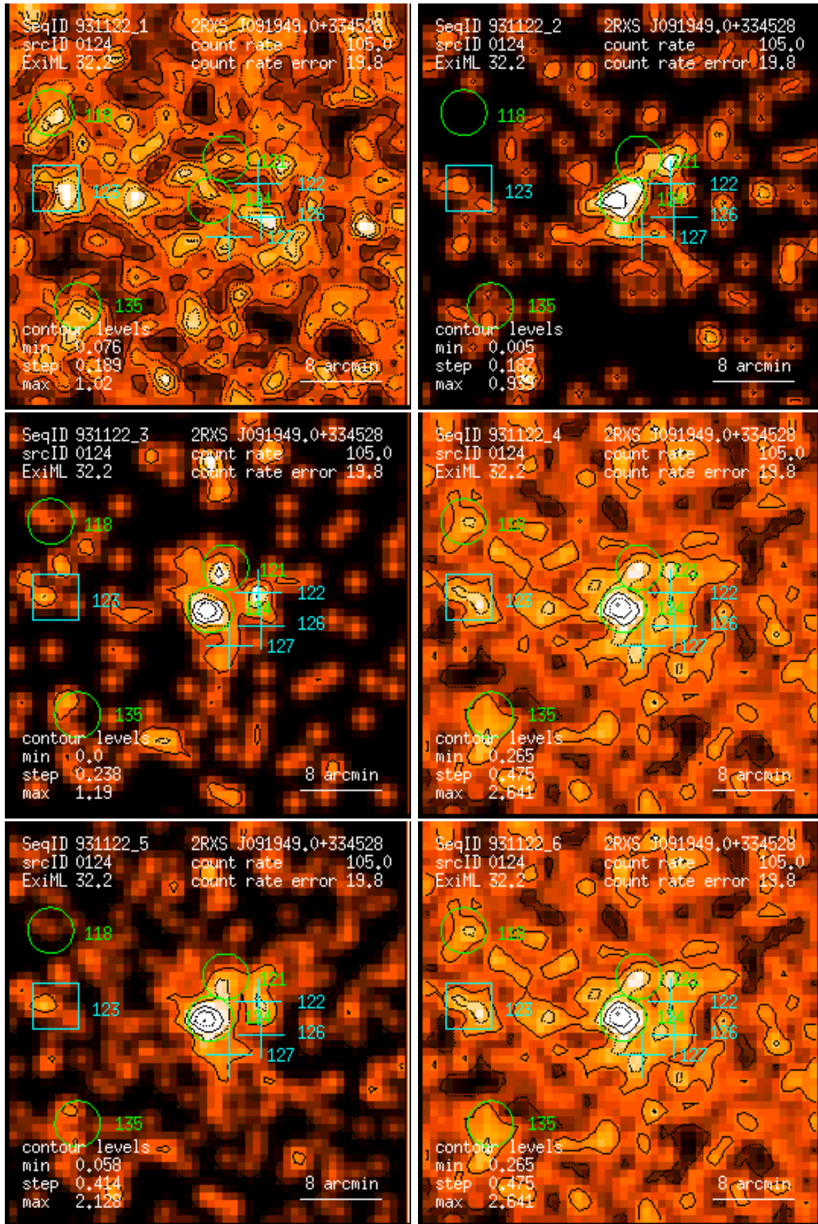
Figure 124: RASS 931122: detection 0124: band rate images, Gaussian filter: (1) PSPC channels 11 – 41, (2) 52 – 90, (3) 91 – 201, (4) 11 – 235, (5) 52 – 201, (6) 11 – 201. Broad band rates in counts/ks. Band rate contour levels in counts/ks/arcmin 2 .
