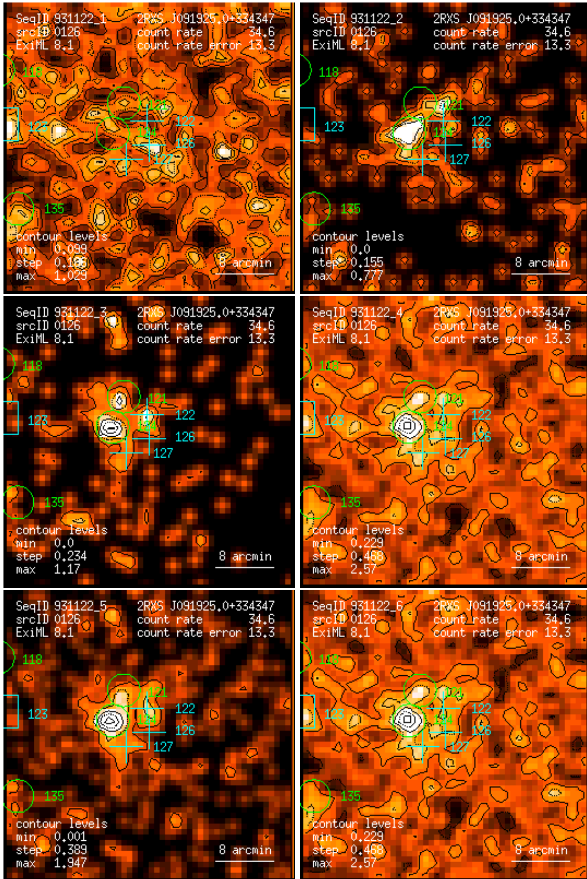
Figure 126: RASS 931122: detection 0126: band rate images, Gaussian filter: (1) PSPC channels 11 – 41, (2) 52 – 90, (3) 91 – 201, (4) 11 – 235, (5) 52 – 201, (6) 11 – 201. Broad band rates in counts/ks. Band rate contour levels in counts/ks/arcmin 2 .
