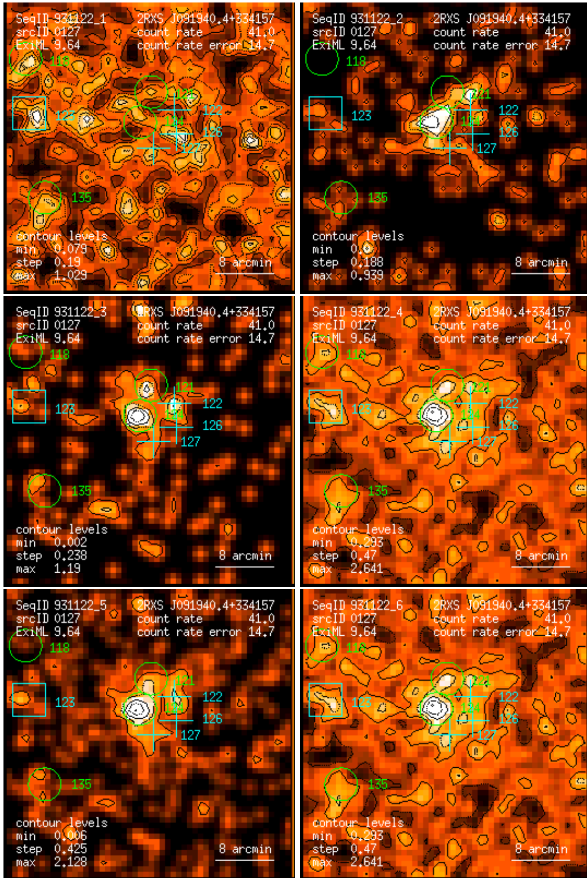
Figure 127: RASS 931122: detection 0127: band rate images, Gaussian filter: (1) PSPC channels 11 – 41, (2) 52 – 90, (3) 91 – 201, (4) 11 – 235, (5) 52 – 201, (6) 11 – 201. Broad band rates in counts/ks. Band rate contour levels in counts/ks/arcmin 2 .
