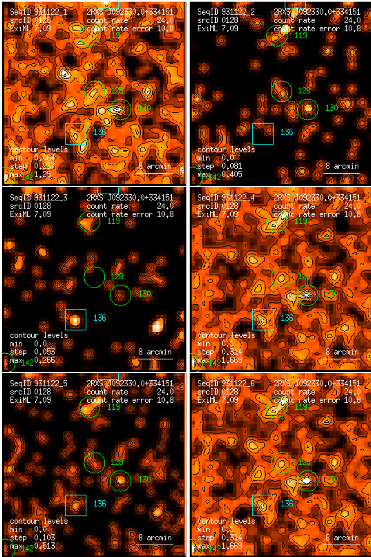
Figure 128: RASS 931122: detection 0128: band rate images, Gaussian filter: (1) PSPC channels 11 – 41, (2) 52 – 90, (3) 91 – 201, (4) 11 – 235, (5) 52 – 201, (6) 11 – 201. Broad band rates in counts/ks. Band rate contour levels in counts/ks/arcmin 2 .
