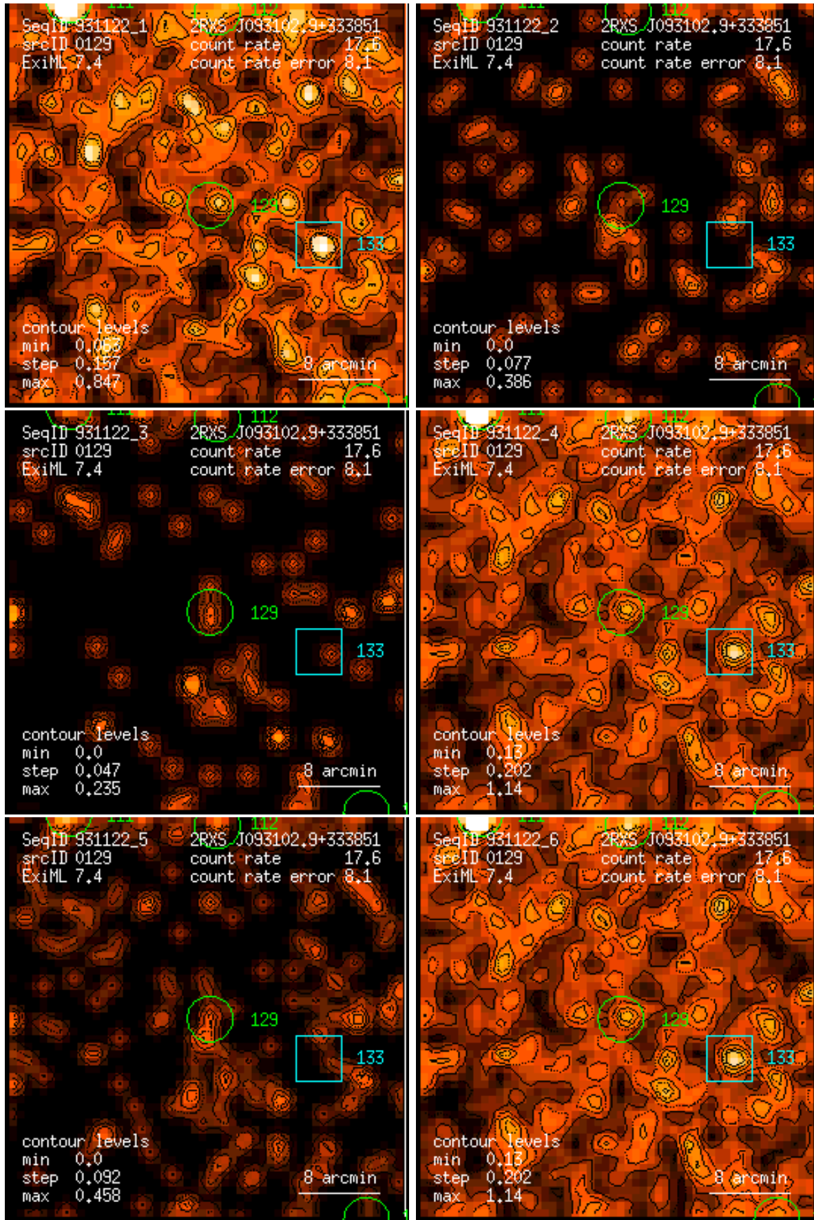
Figure 129: RASS 931122: detection 0129: band rate images, Gaussian filter: (1) PSPC channels 11 – 41, (2) 52 – 90, (3) 91 – 201, (4) 11 – 235, (5) 52 – 201, (6) 11 – 201. Broad band rates in counts/ks. Band rate contour levels in counts/ks/arcmin 2 .
