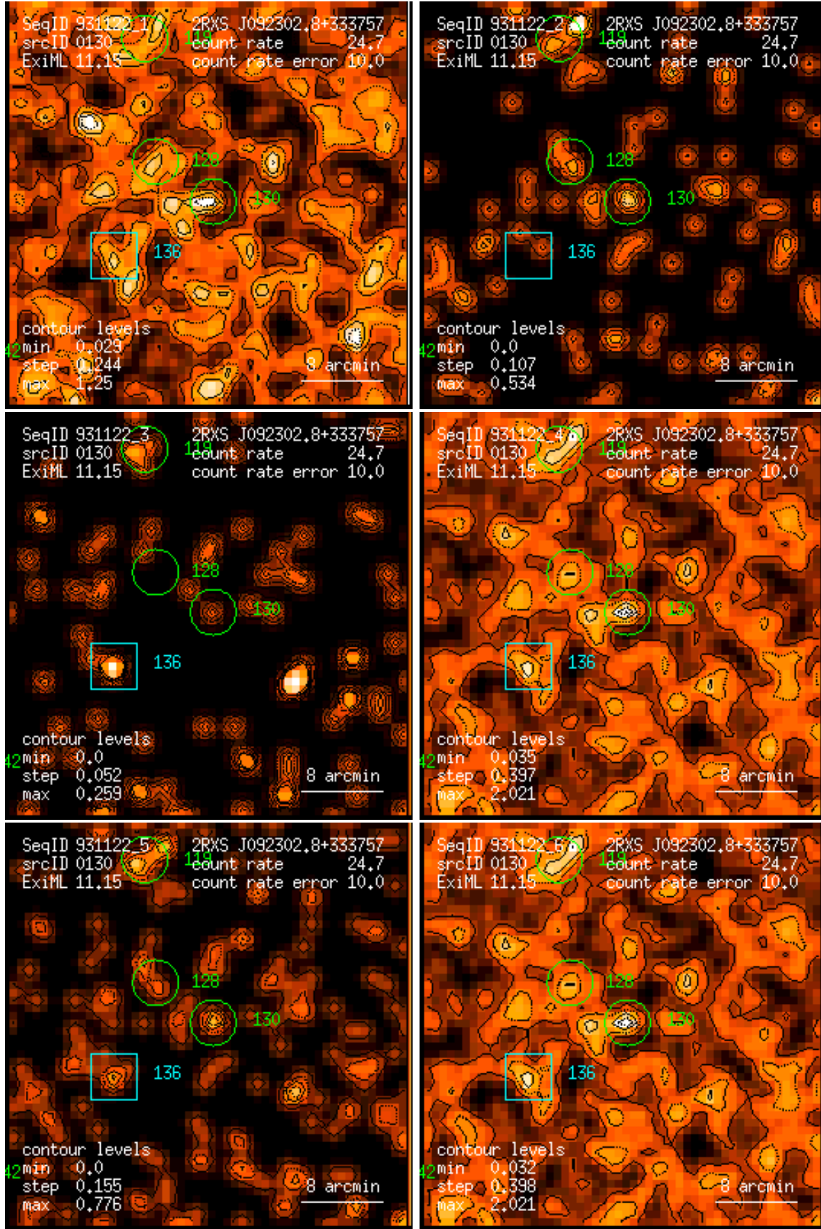
Figure 130: RASS 931122: detection 0130: band rate images, Gaussian filter: (1) PSPC channels 11 – 41, (2) 52 – 90, (3) 91 – 201, (4) 11 – 235, (5) 52 – 201, (6) 11 – 201. Broad band rates in counts/ks. Band rate contour levels in counts/ks/arcmin 2 .
