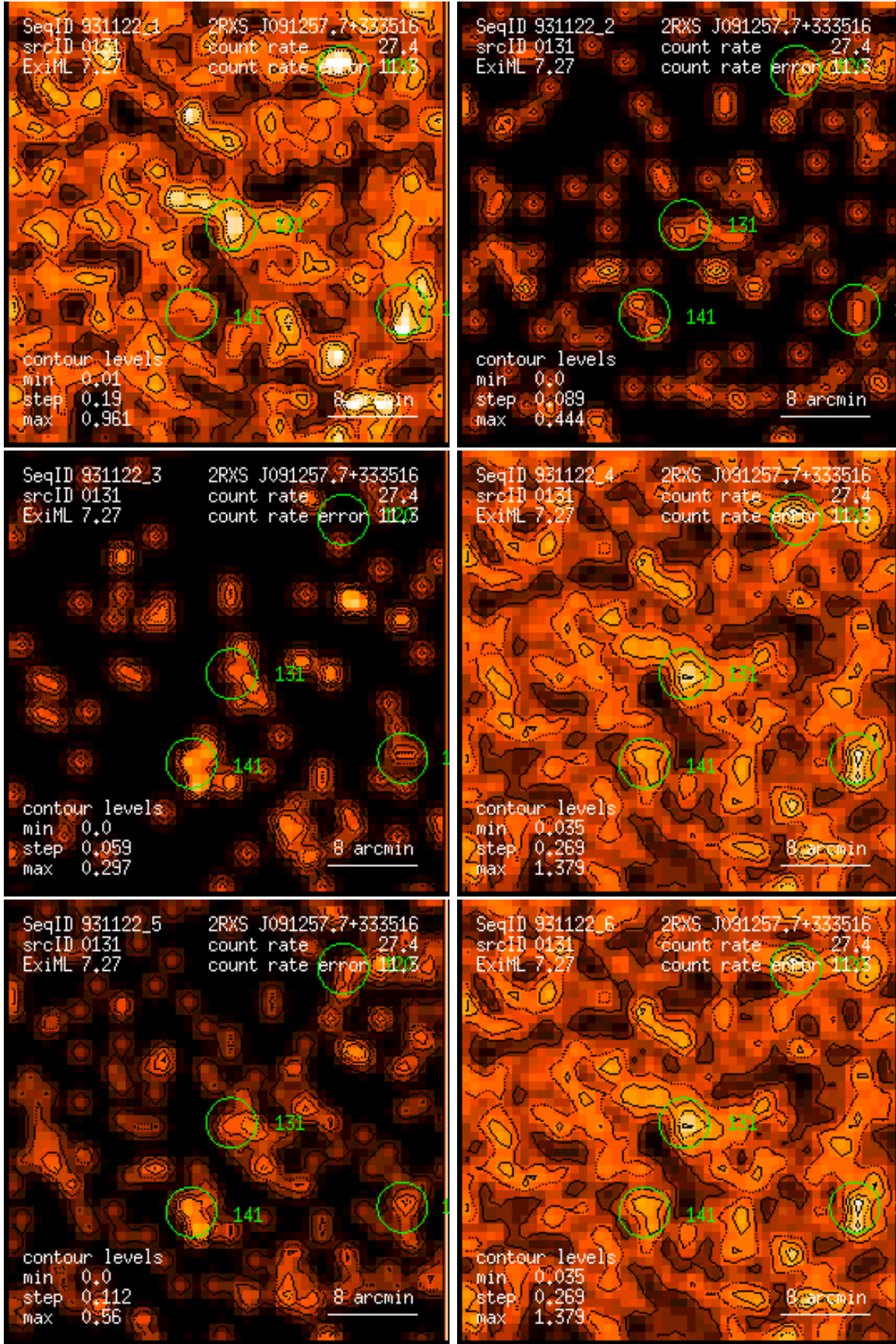
Figure 131: RASS 931122: detection 0131: band rate images, Gaussian filter: (1) PSPC channels 11 – 41, (2) 52 – 90, (3) 91 – 201, (4) 11 – 235, (5) 52 – 201, (6) 11 – 201. Broad band rates in counts/ks. Band rate contour levels in counts/ks/arcmin 2 .
