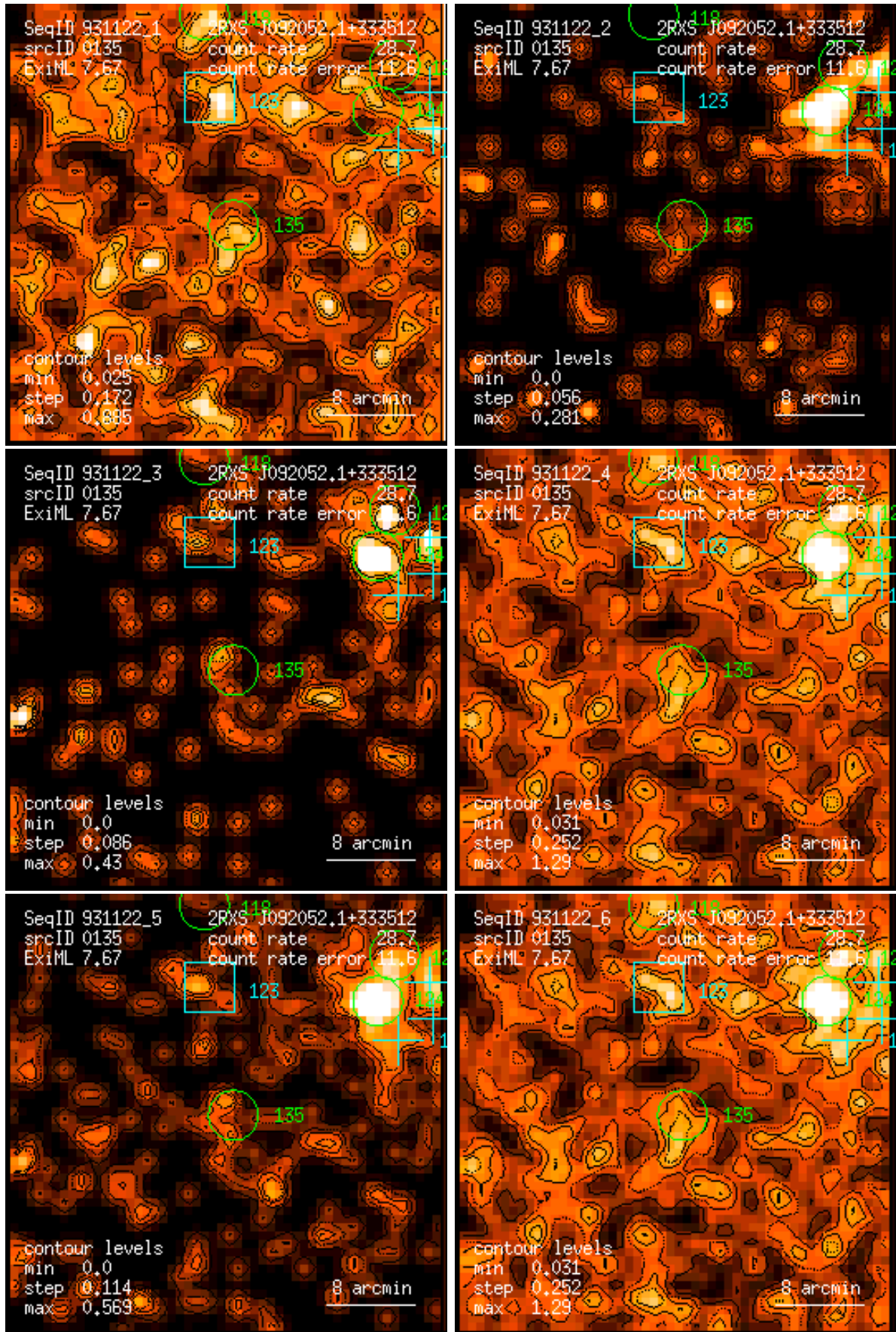
Figure 135: RASS 931122: detection 0135: band rate images, Gaussian filter: (1) PSPC channels 11 – 41, (2) 52 – 90, (3) 91 – 201, (4) 11 – 235, (5) 52 – 201, (6) 11 – 201. Broad band rates in counts/ks. Band rate contour levels in counts/ks/arcmin 2 .
