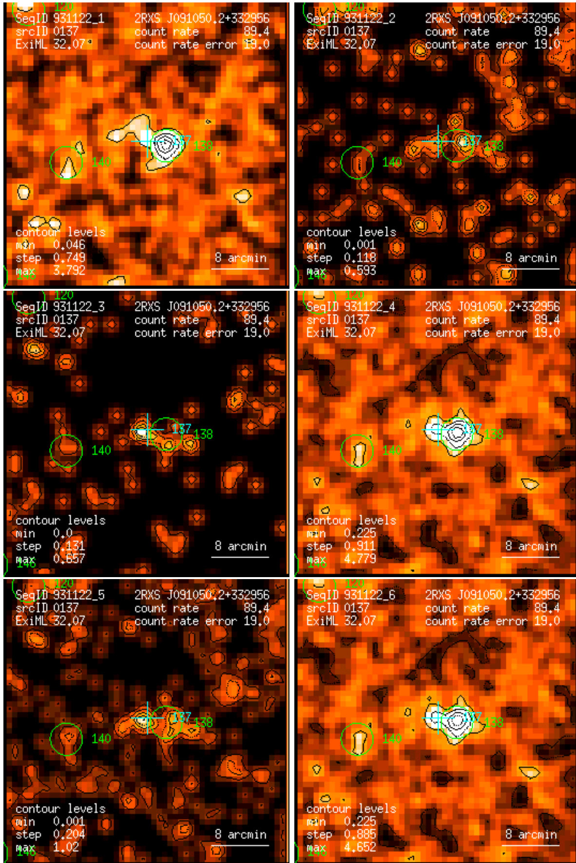
Figure 137: RASS 931122: detection 0137: band rate images, Gaussian filter: (1) PSPC channels 11 – 41, (2) 52 – 90, (3) 91 – 201, (4) 11 – 235, (5) 52 – 201, (6) 11 – 201. Broad band rates in counts/ks. Band rate contour levels in counts/ks/arcmin 2 .
