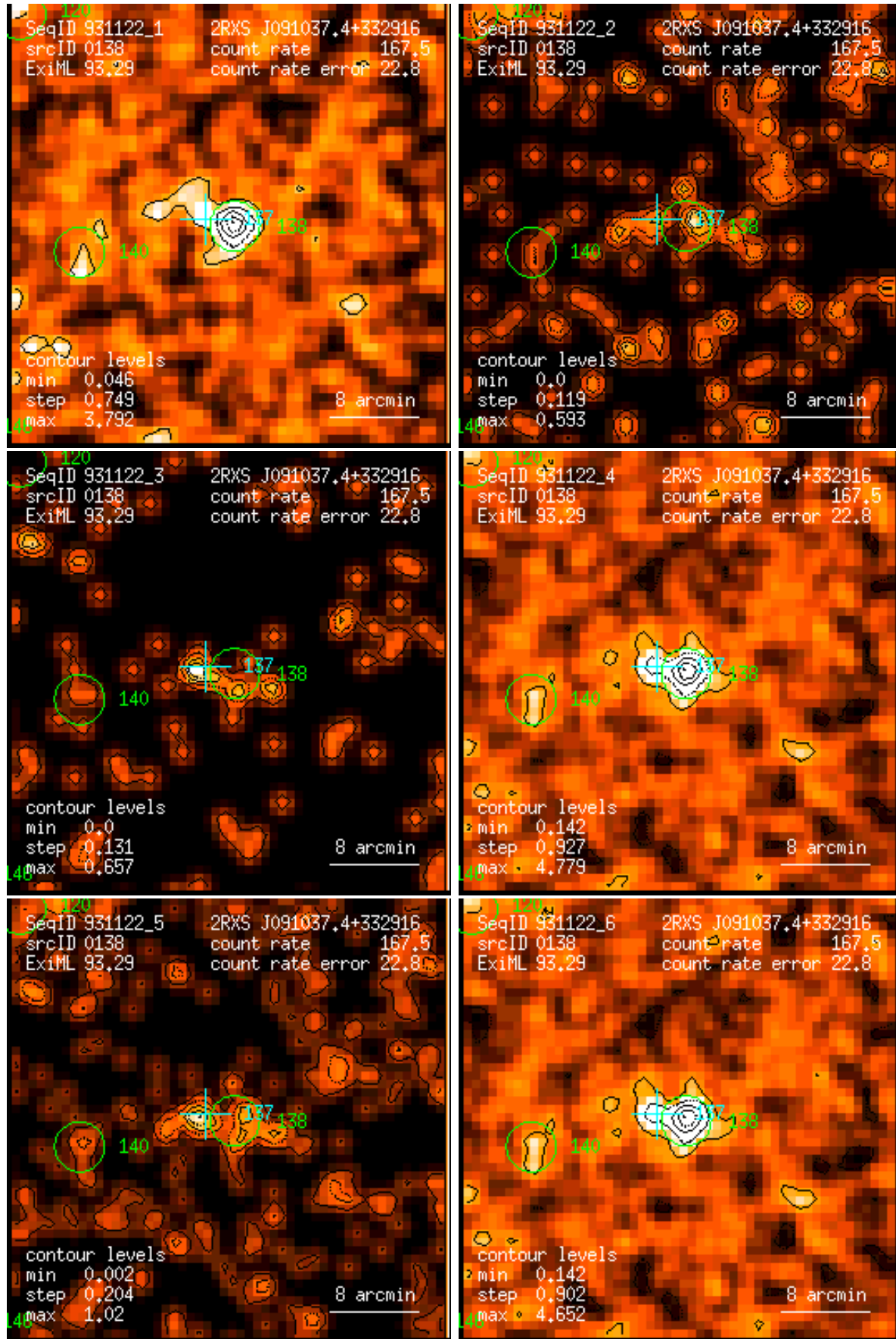
Figure 138: RASS 931122: detection 0138: band rate images, Gaussian filter: (1) PSPC channels 11 – 41, (2) 52 – 90, (3) 91 – 201, (4) 11 – 235, (5) 52 – 201, (6) 11 – 201. Broad band rates in counts/ks. Band rate contour levels in counts/ks/arcmin 2 .
