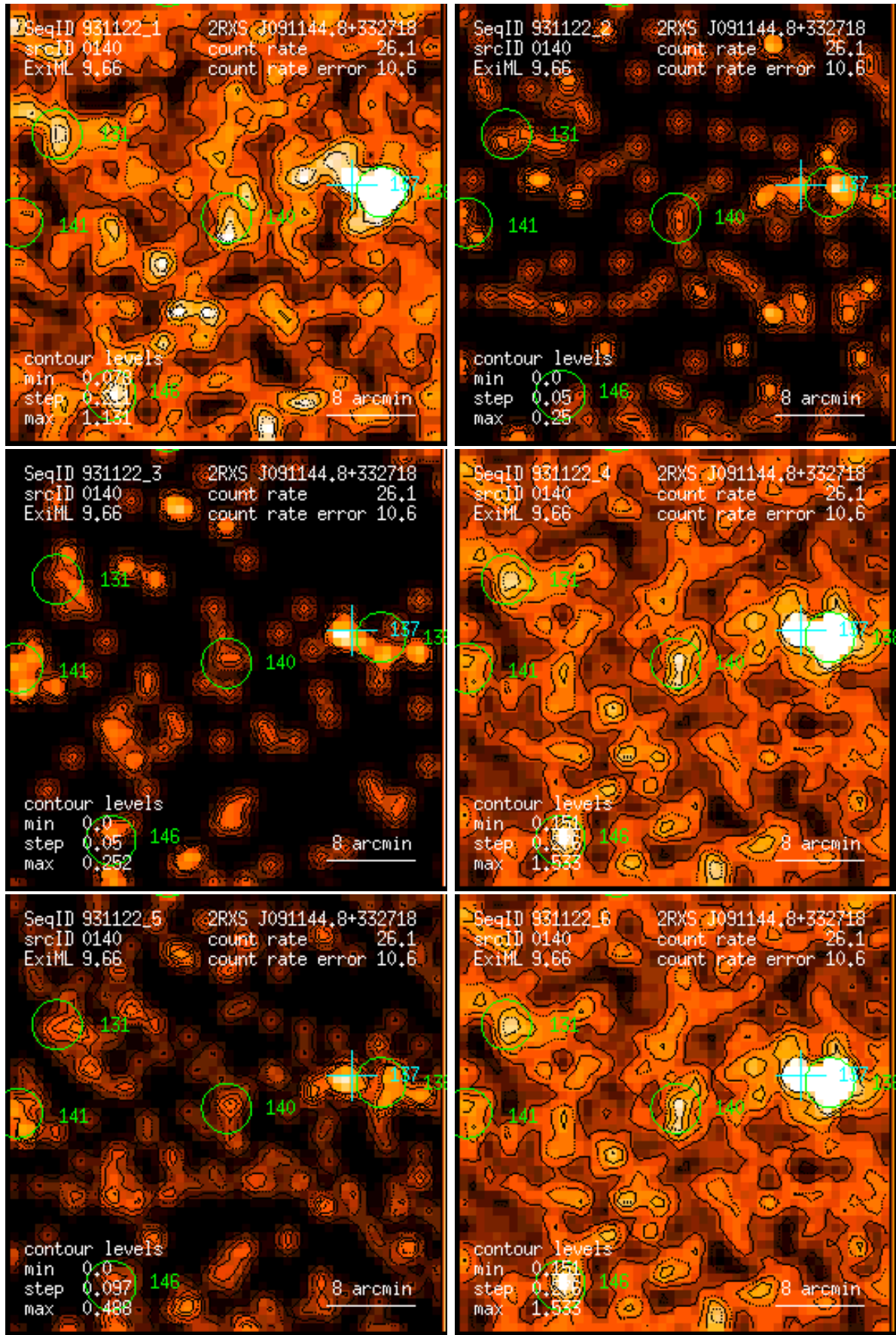
Figure 140: RASS 931122: detection 0140: band rate images, Gaussian filter: (1) PSPC channels 11 – 41, (2) 52 – 90, (3) 91 – 201, (4) 11 – 235, (5) 52 – 201, (6) 11 – 201. Broad band rates in counts/ks. Band rate contour levels in counts/ks/arcmin 2 .
