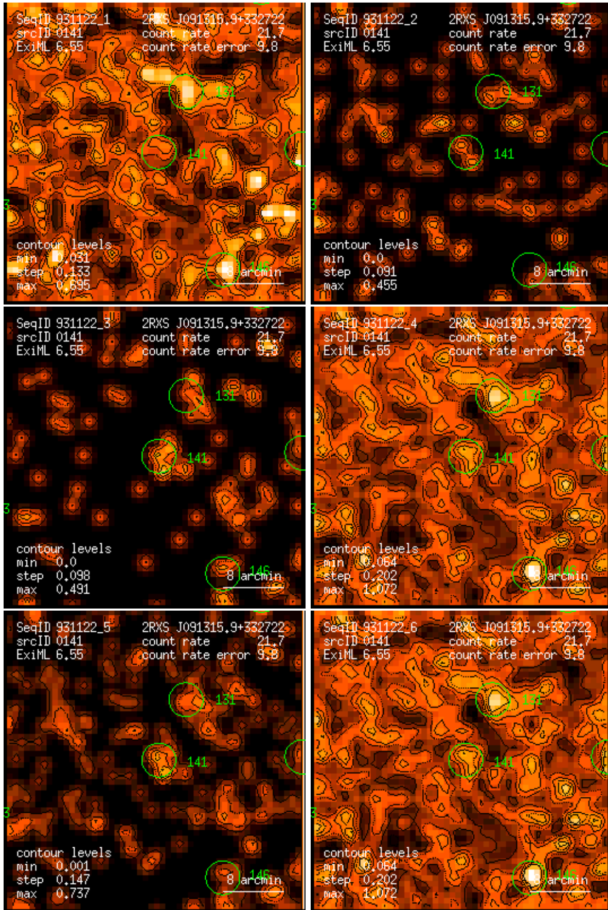
Figure 141: RASS 931122: detection 0141: band rate images, Gaussian filter: (1) PSPC channels 11 – 41, (2) 52 – 90, (3) 91 – 201, (4) 11 – 235, (5) 52 – 201, (6) 11 – 201. Broad band rates in counts/ks. Band rate contour levels in counts/ks/arcmin 2 .
