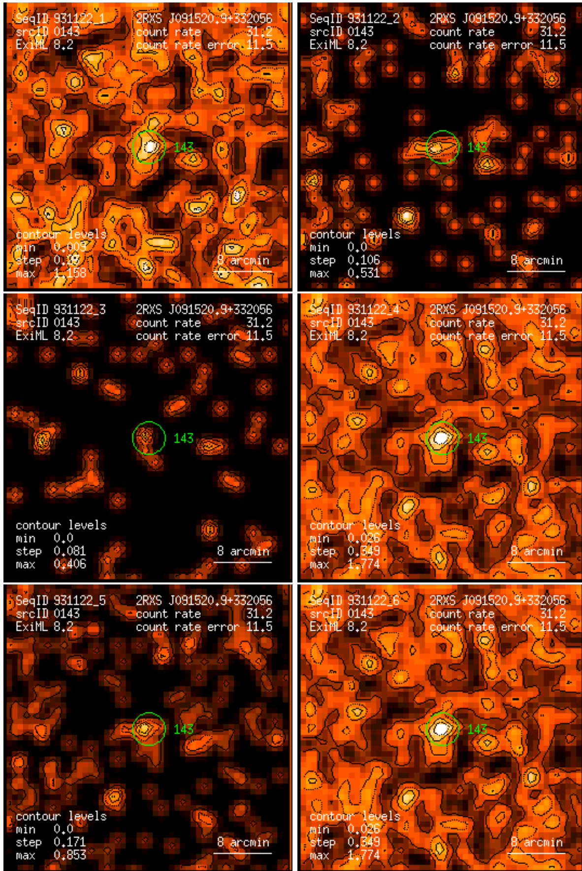
Figure 143: RASS 931122: detection 0143: band rate images, Gaussian filter: (1) PSPC channels 11 – 41, (2) 52 – 90, (3) 91 – 201, (4) 11 – 235, (5) 52 – 201, (6) 11 – 201. Broad band rates in counts/ks. Band rate contour levels in counts/ks/arcmin 2 .
