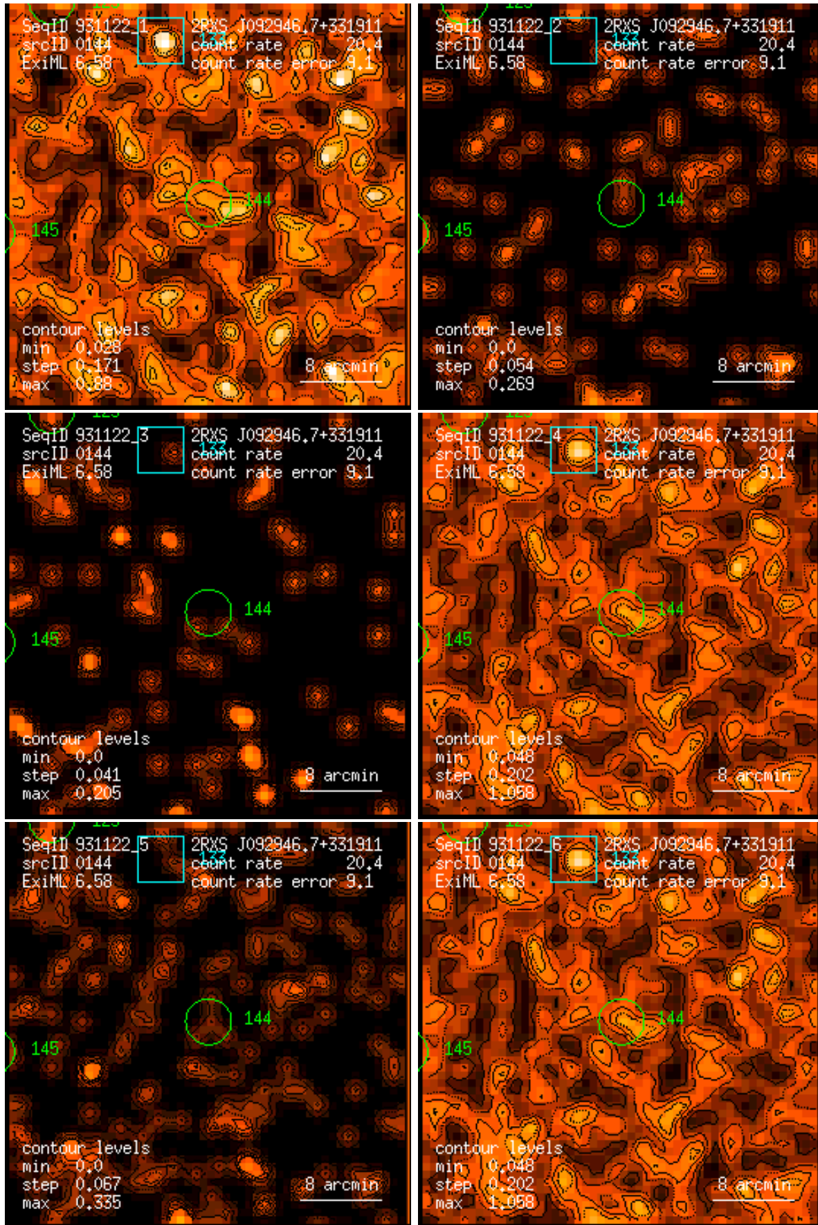
Figure 144: RASS 931122: detection 0144: band rate images, Gaussian filter: (1) PSPC channels 11 – 41, (2) 52 – 90, (3) 91 – 201, (4) 11 – 235, (5) 52 – 201, (6) 11 – 201. Broad band rates in counts/ks. Band rate contour levels in counts/ks/arcmin 2 .
