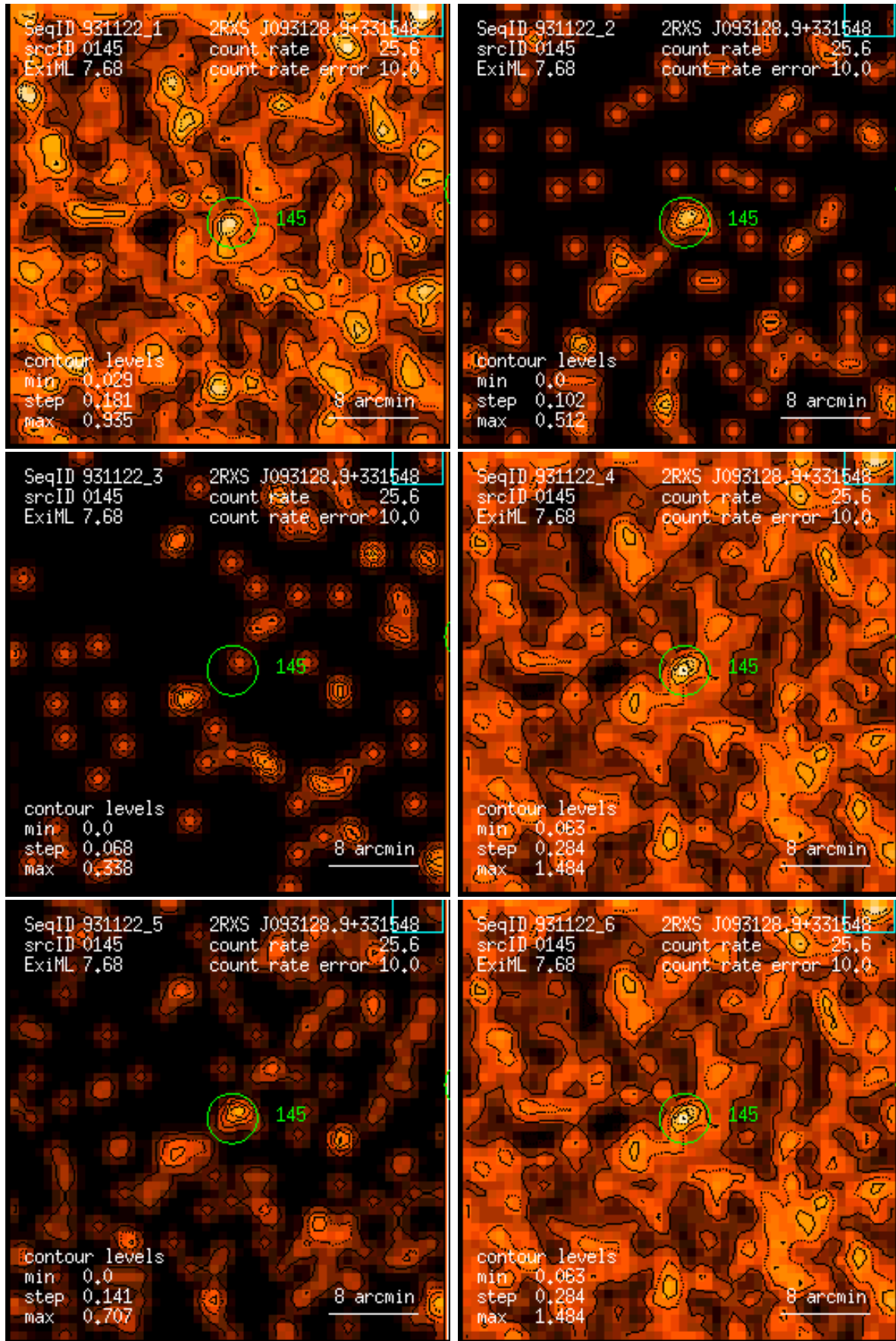
Figure 145: RASS 931122: detection 0145: band rate images, Gaussian filter: (1) PSPC channels 11 – 41, (2) 52 – 90, (3) 91 – 201, (4) 11 – 235, (5) 52 – 201, (6) 11 – 201. Broad band rates in counts/ks. Band rate contour levels in counts/ks/arcmin 2 .
