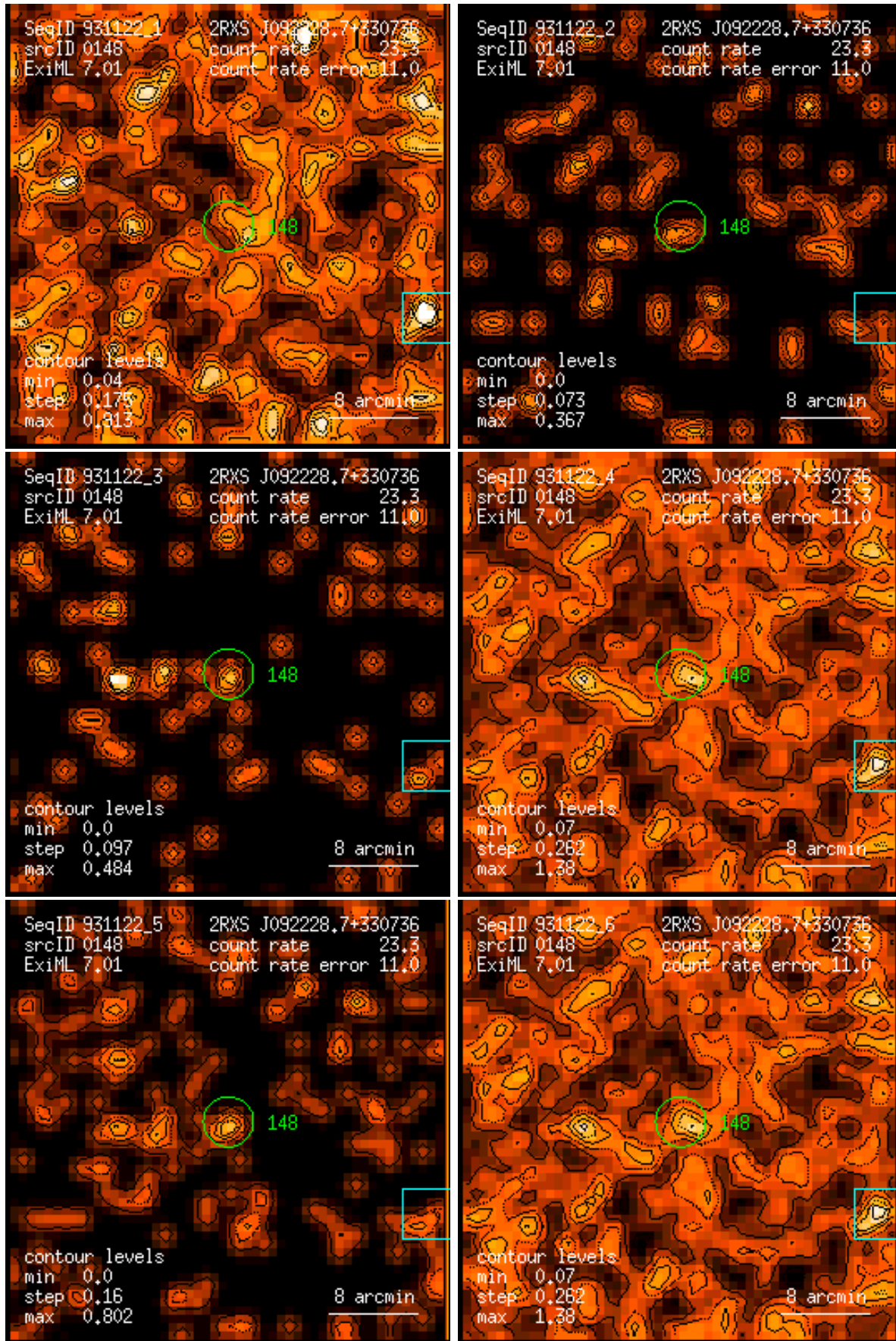
Figure 148: RASS 931122: detection 0148: band rate images, Gaussian filter: (1) PSPC channels 11 – 41, (2) 52 – 90, (3) 91 – 201, (4) 11 – 235, (5) 52 – 201, (6) 11 – 201. Broad band rates in counts/ks. Band rate contour levels in counts/ks/arcmin 2 .
