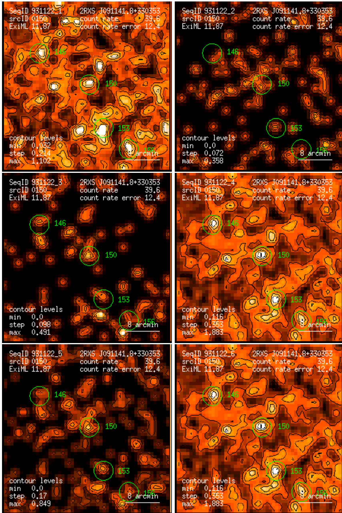
Figure 150: RASS 931122: detection 0150: band rate images, Gaussian filter: (1) PSPC channels 11 – 41, (2) 52 – 90, (3) 91 – 201, (4) 11 – 235, (5) 52 – 201, (6) 11 – 201. Broad band rates in counts/ks. Band rate contour levels in counts/ks/arcmin 2 .
