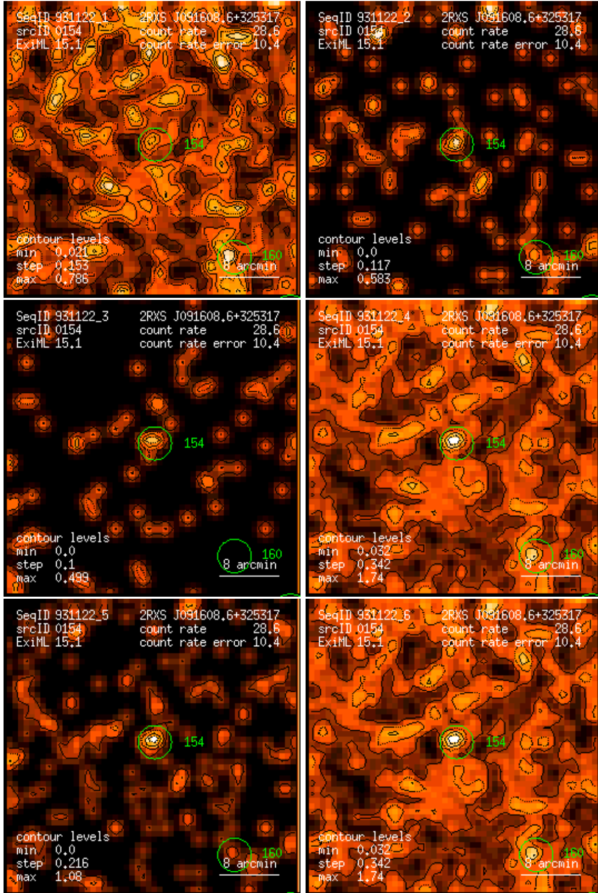
Figure 154: RASS 931122: detection 0154: band rate images, Gaussian filter: (1) PSPC channels 11 – 41, (2) 52 – 90, (3) 91 – 201, (4) 11 – 235, (5) 52 – 201, (6) 11 – 201. Broad band rates in counts/ks. Band rate contour levels in counts/ks/arcmin 2 .
