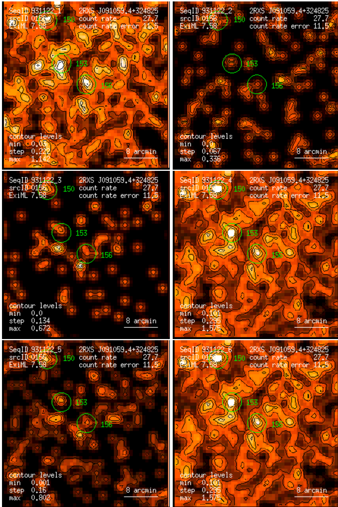
Figure 156: RASS 931122: detection 0156: band rate images, Gaussian filter: (1) PSPC channels 11 – 41, (2) 52 – 90, (3) 91 – 201, (4) 11 – 235, (5) 52 – 201, (6) 11 – 201. Broad band rates in counts/ks. Band rate contour levels in counts/ks/arcmin 2 .
