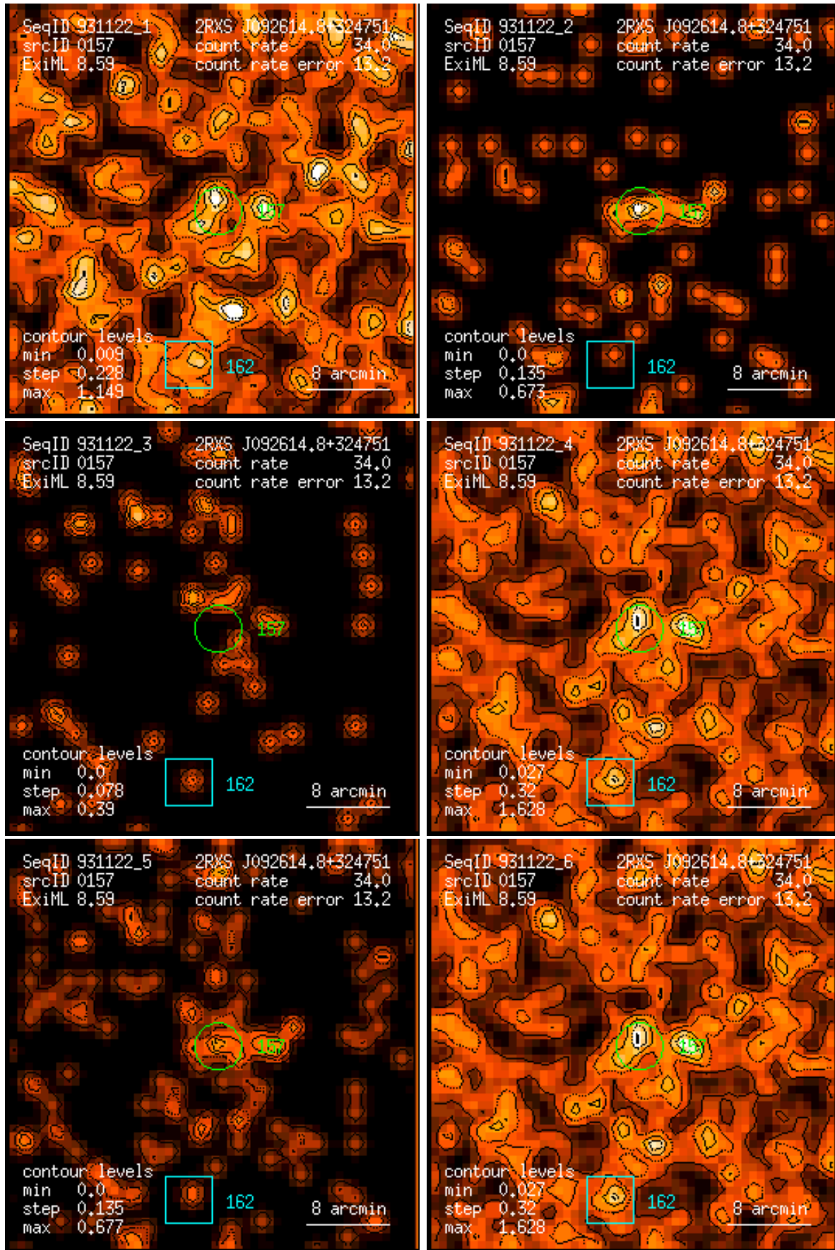
Figure 157: RASS 931122: detection 0157: band rate images, Gaussian filter: (1) PSPC channels 11 – 41, (2) 52 – 90, (3) 91 – 201, (4) 11 – 235, (5) 52 – 201, (6) 11 – 201. Broad band rates in counts/ks. Band rate contour levels in counts/ks/arcmin 2 .
