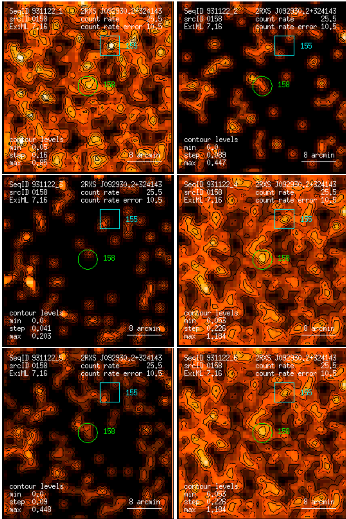
Figure 158: RASS 931122: detection 0158: band rate images, Gaussian filter: (1) PSPC channels 11 – 41, (2) 52 – 90, (3) 91 – 201, (4) 11 – 235, (5) 52 – 201, (6) 11 – 201. Broad band rates in counts/ks. Band rate contour levels in counts/ks/arcmin 2 .
