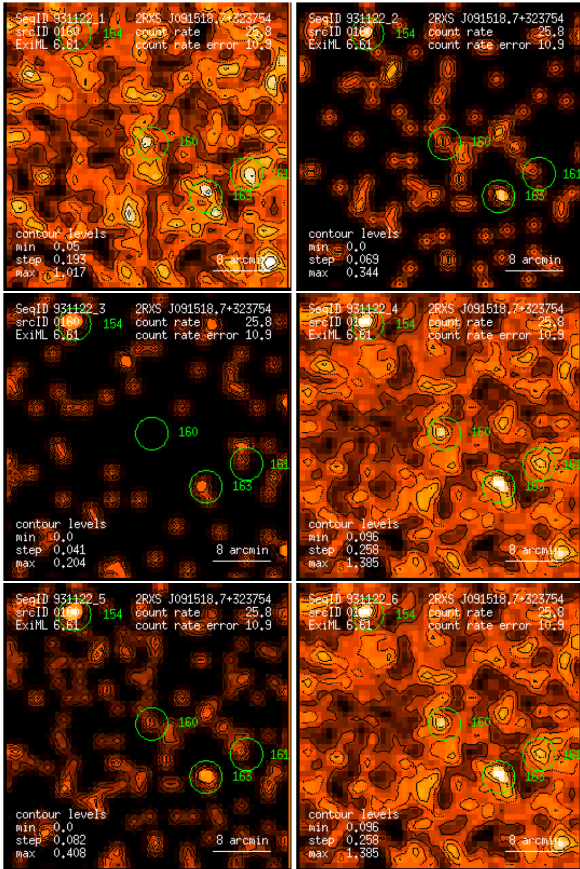
Figure 160: RASS 931122: detection 0160: band rate images, Gaussian filter: (1) PSPC channels 11 – 41, (2) 52 – 90, (3) 91 – 201, (4) 11 – 235, (5) 52 – 201, (6) 11 – 201. Broad band rates in counts/ks. Band rate contour levels in counts/ks/arcmin 2 .
