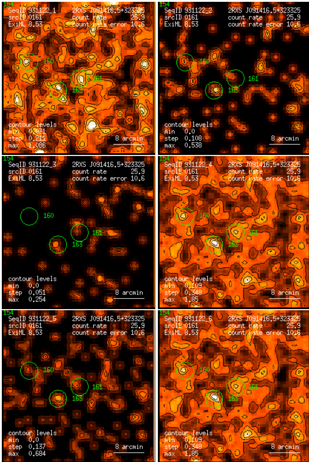
Figure 161: RASS 931122: detection 0161: band rate images, Gaussian filter: (1) PSPC channels 11 – 41, (2) 52 – 90, (3) 91 – 201, (4) 11 – 235, (5) 52 – 201, (6) 11 – 201. Broad band rates in counts/ks. Band rate contour levels in counts/ks/arcmin 2 .
